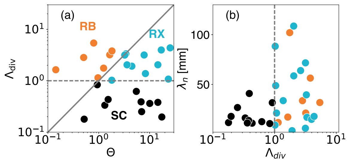
Figure 13: (a) \Lambda_{div} vs \Theta plot. The orange and blue points are those where, according to [1], the blobs should be electrically disconnected
