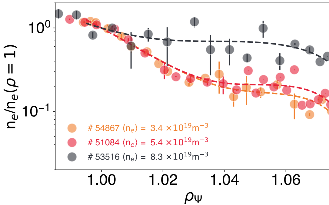
Figure 2: Upstream density profile normalized to the value at the separatrix obtained in similar L-Mode, LSN discharges at 3 values of density
