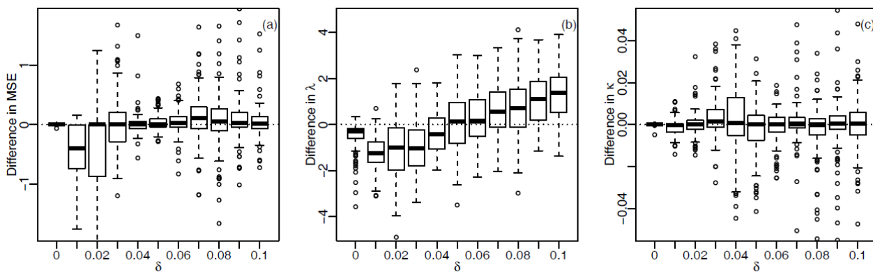
Fig. 13. Wavelet then inversion results, with joint estimation of parameters, showing boxplots improvement due to simultaneous estimation: (a) MSE and estimated parameters (b) \lambda and (c) \kappa - a negative value indicates a higher value for sequential estimation
