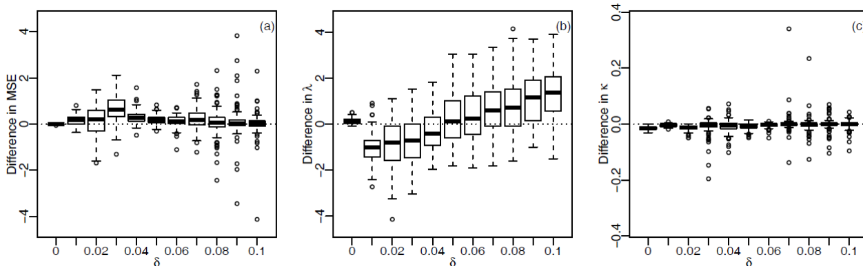
Fig. 11. Comparison of Method 1 and Method 2 with sequential estimation of parameters - a negative value indicates that Method 1 has a higher value.
