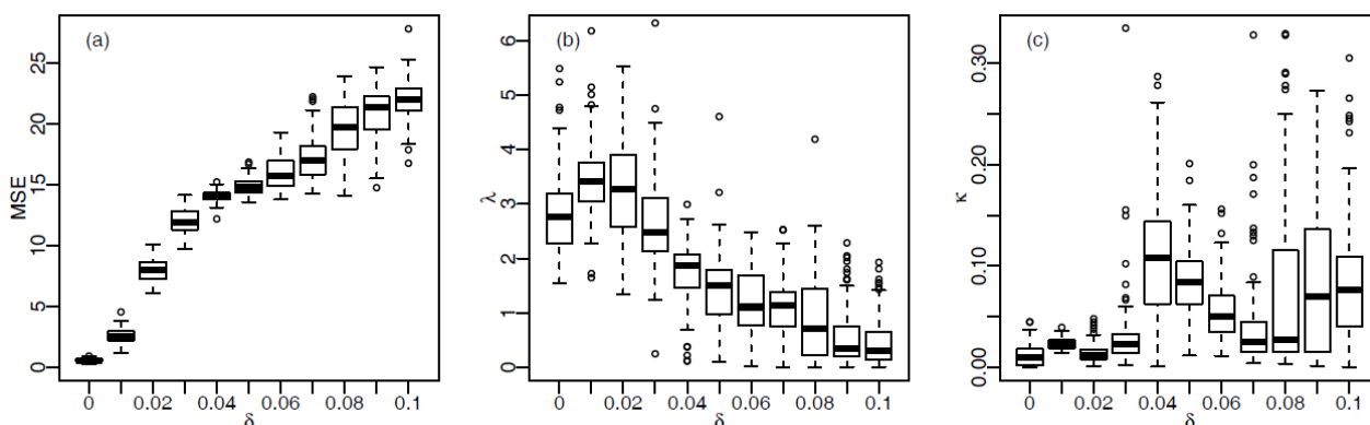
Fig. 12. Wavelet then inversion results, with joint estimation of parameters, showing boxplots: (a) MSE and estimated parameters (b) \lambda and (c) \kappa
