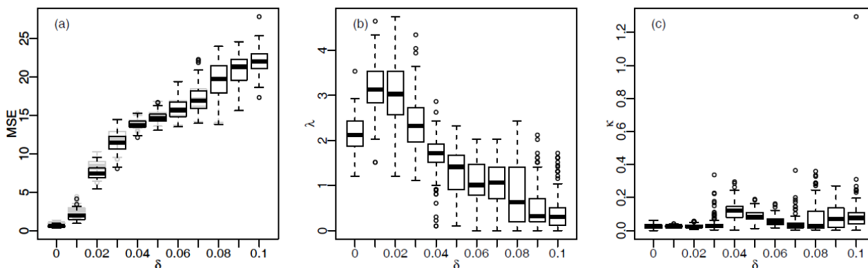
Fig. 10. Inversion then wavelet results showing boxplots: (a) MSE after inversion (grey) and then after thresholding (black) and estimated parameters (b) \hat{\lambda} and (c) \hat{\kappa}
