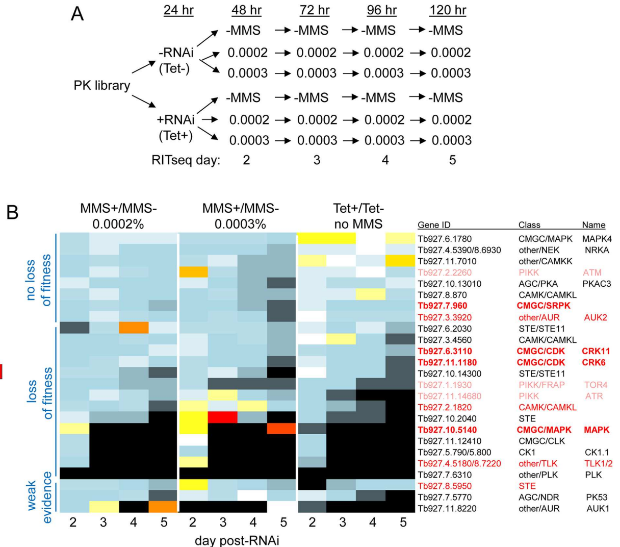
Fig 6. A kinome-focused MMS RIT-seq screen. A. A pool (library) of BSF T. brucei cells was generated allowing parallel tetracycline (Tet) induction of RNAi against all protein kinase (PK) genes. The pool was split, RNAi initiated in one culture (Tet+) and the other grown without RNAi (Tet-). After 24 hrs both cultures were further split and grown for four days in the presence of either 0.0002% or 0.0003% MMS, or without addition of damaging agent (MMS-). DNA was prepared from the populations on days 2, 3, 4 and 5 and PCR used to recover the PK-specific RNAi targets. PCR products were sequenced and mapped to the PK genes, determining read abundance in the different conditions and at different times. B. A heatmap of ratios of reads in the different populations shown in A are detailed for putative MMS damage response PK genes, which are identified by gene ID, PK class and name (if known); all PK genes are provided in S4 Table . For each gene MMS+/MMS- ratios are shown at each of the 4 days examined and at both MMS concentrations; to evaluate the importance of the genes for cell survival, ratios of RNAi target reads from the Tet+ cells relative to the Tet- cells, without addition of MMS, are shown at the same time points. Genes highlighted in bold red were not seen in the genome-wide MMS RIT-seq but were validated by targeted RNAi ( Fig 7 ); genes in red are common between the two MMS RIT-seq screens; and genes in pink have predicted roles in MMS damage repair in other eukaryotes.
