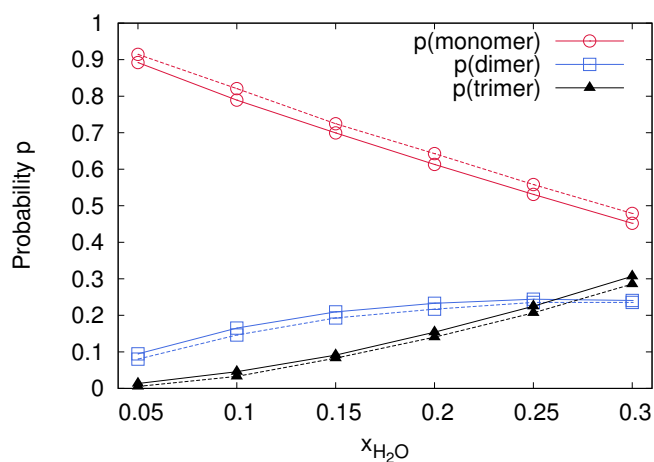
Fig. 10 Probability of water molecules in monomeric p(monomer), dimeric p(dimer) and trimeric/tetrameric p(trimer) arrangement in EMIM/BF4 (solid line) and BMIM/BF4 (dashed line) for different water mole fractions.
