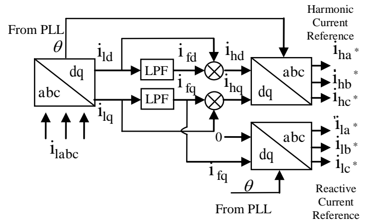
Fig. 10. STATCOM Current Control Scheme
