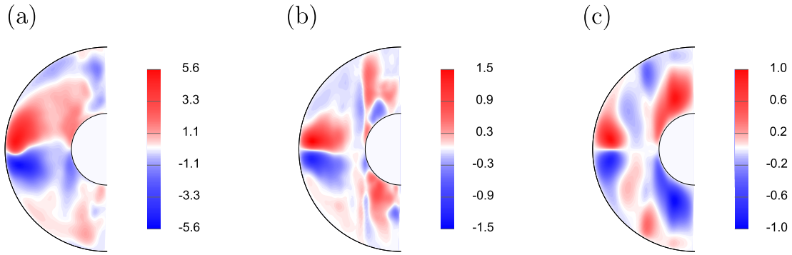
Fig. 2. Meridional plots of time-averaged axisymmetric azimuthal field \overline{B_\phi^s} for models 4R5 (a), 6.5R2 (b), and 4R2 (c).
