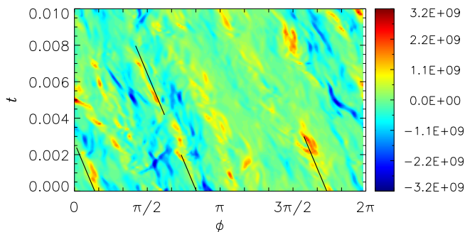
Fig. 11. A sum of dominant restoring and nonlinear Lorentz terms, \overline{P_m^E} \left( \frac{B_s + B_s'}{s} \frac{\partial f}{\partial \phi} \right) , at r = 0.5r_o for the dynamo run 5R5. Narrow waveforms observed in \Xi_C or \langle u_s' \rangle are somehow reproduced.
