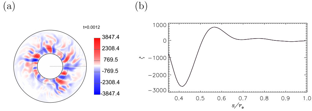
Fig. 7. Spatial structures of (a) z-averaged radial velocity ( u_s ) (cf. Fig. 3a) and (b) angular velocity \zeta (cf. Fig. 1b of HJT15) for nonmagnetic model NM_5R5.
