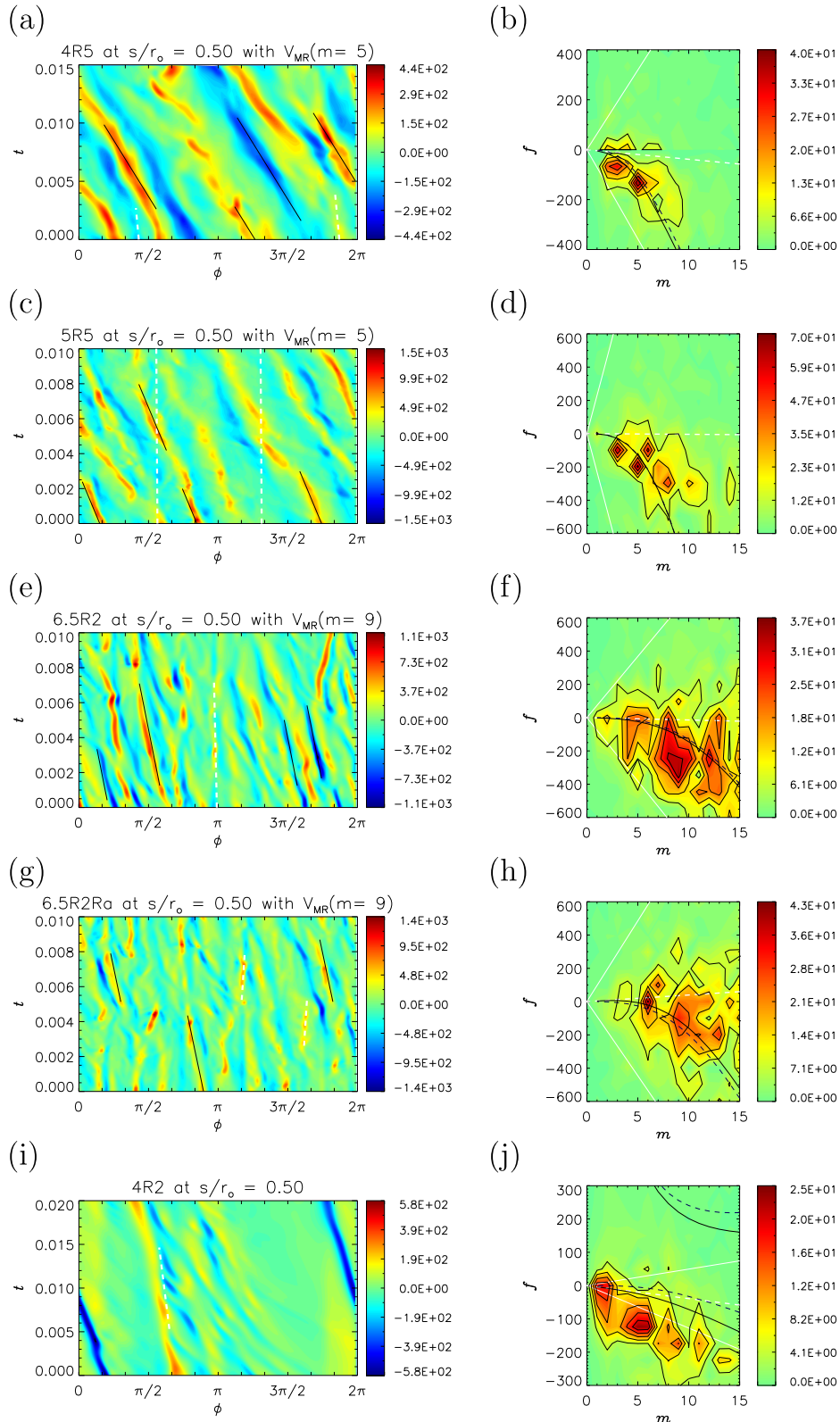
Fig. 4. The radial velocity, \langle u'_s \rangle , at radius s = 0.5r_o for models 4R5 (a-b), 5R5 (c-d), 6.5R2 (e-f), 6.5R2Ra (g-h), and 4R2 (i-j). (Left) Azimuth-time section. White dashed and black solid lines represent the advective speeds, \zeta , and the total speeds of advection and MR wave propagation, \zeta + \hat{\omega}_{MR}/m , respectively. (Right) Wavenumber-frequency power spectrum. White dashed, black dashed, black solid, and white solid lines represent the dispersion relations of advection ( \omega_{adv}/2\pi ), waves ( \hat{\omega}_{\pm}/2\pi ), advection plus waves ( (\omega_{adv} + \hat{\omega}_{\pm})/2\pi ), and advection plus Alfvén waves ( (\omega_{adv} \pm \hat{\omega}_M)/2\pi ), respectively.
