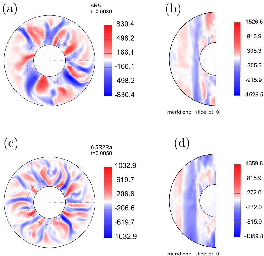
Fig. 3. (Left) Spatial structures of \langle u_s \rangle and (right) meridional slices of u_s at zero longitude for models 5R5 (a-b) and 6.5R2Ra (c-d). Each snapshot is taken at the time shown in the figure. In the left column, dotted lines indicate the radius s = 0.5r_o and the longitude \phi = 0 .
