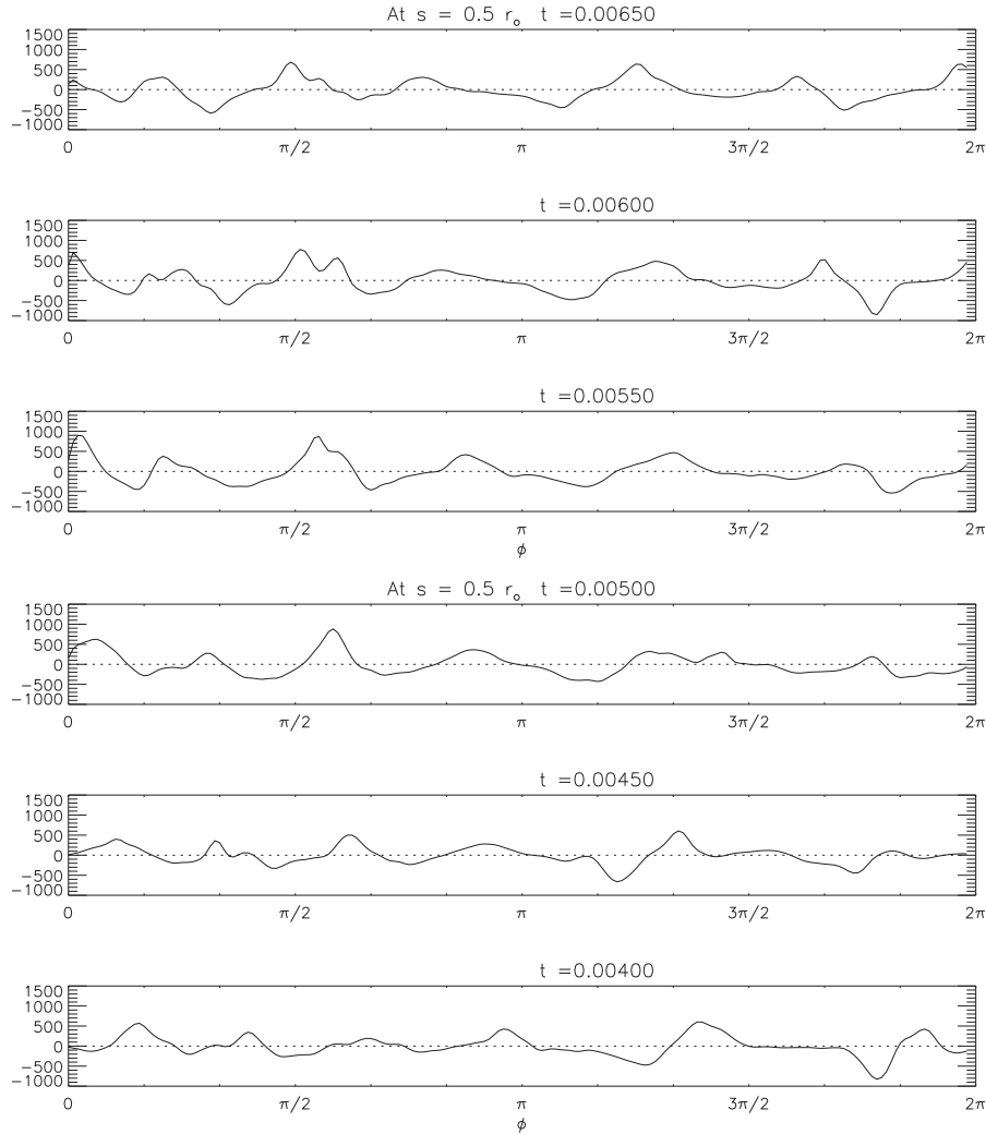
Fig. 5. Time evolution of \langle u'_\phi \rangle at s = 0.5r_o for model 5R5 (cf. Fig. 4c). Time evolves from bottom to top.
