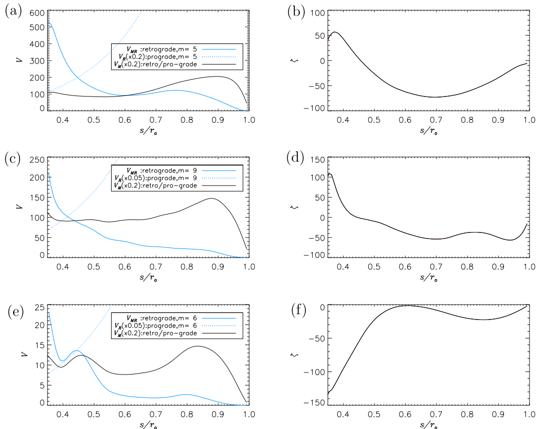
Fig. 1. (Left) Phase speeds of waves propagating in azimuth and (right) angular velocity, \zeta = \langle \overline{U_\phi} \rangle / s , as a function of s/r_o . From top to bottom, models 4R5 (a–b), 6.5R2 (c–d), and 4R2 (e–f) are shown. In the left column blue solid, blue dotted, and black solid curves represent magnetic Rossby, V_{MR} = |\hat{\omega}_{MR}/m| , (nonmagnetic) Rossby, V_R = |\hat{\omega}_R/m| , and Alfvén, V_M = |\hat{\omega}_M/m| , waves, respectively. Each legend presents the wavenumber m used to calculate V_{MR} and V_R and the factor used to rescale V_R and V_M . (For interpretation of the references to colour in this figure legend, the reader is referred to the web version of this article.)
