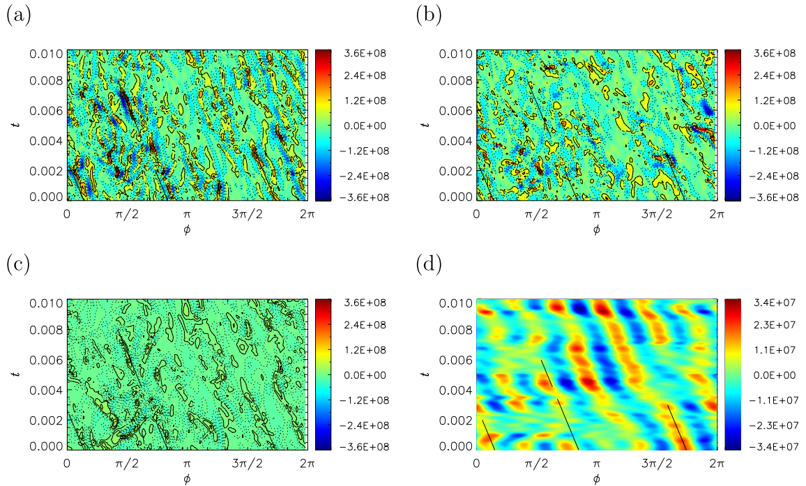
Fig. 10. Azimuth-time section at r = 0.5r_o of the restoring parts of the Lorentz term, \Xi_L , for model 5R5. (a) \overline{P_m^E} \left( \frac{B_s}{s} \frac{\partial f}{\partial \phi} \right) , (b) \overline{P_m^E} \left( B_s \frac{\partial f}{\partial s} \right) , (c) \overline{P_m^E} \left( B_z \frac{\partial f}{\partial z} \right) , and (d) \overline{P_m^E} \left( \frac{B_s}{s} \frac{\partial f}{\partial \phi} \right) bandpass filtered over m = 4 to 6.
