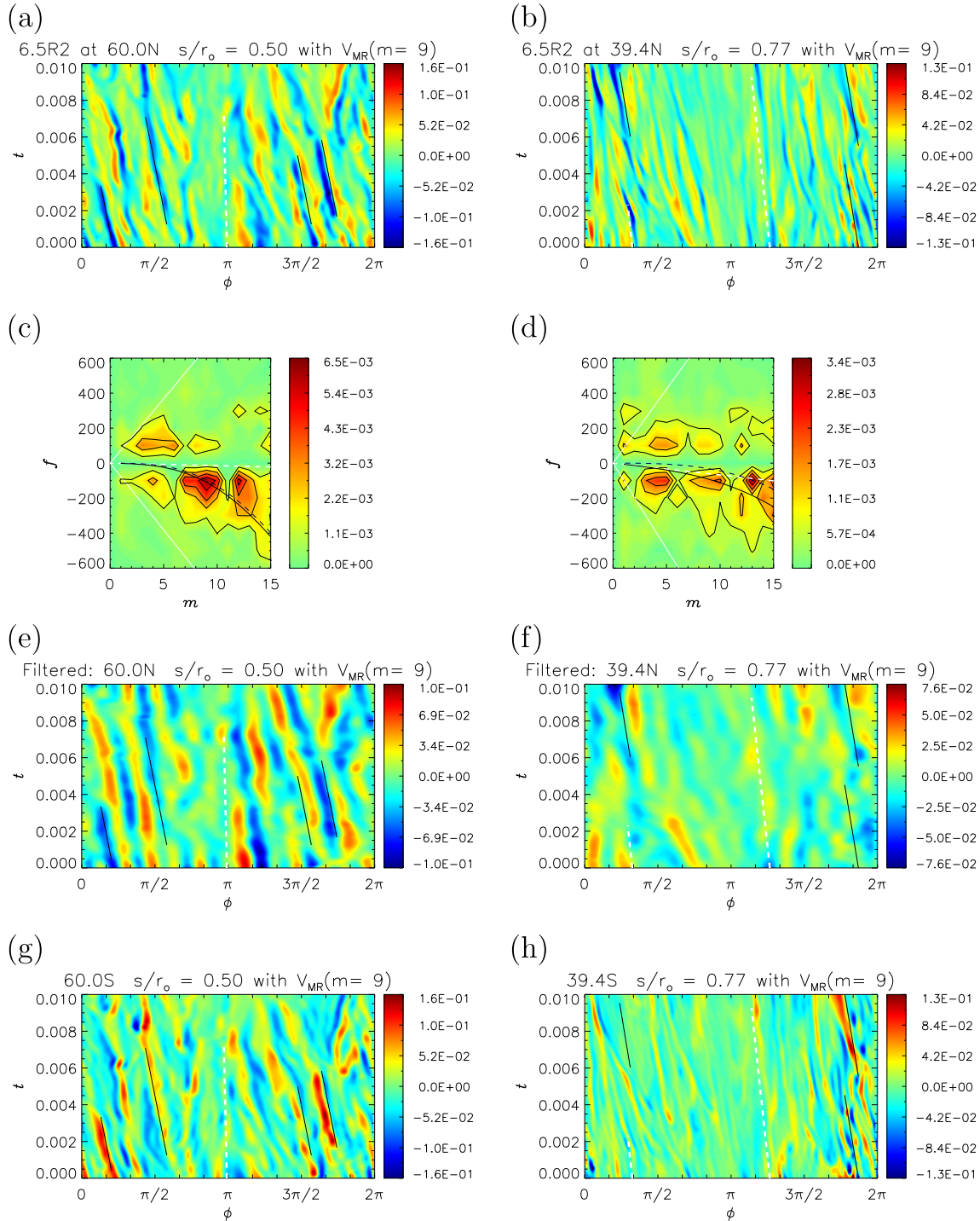
Fig. 12. The residual part B_r' of the radial magnetic field at r = r_o at different latitudes for run 6.5R2. (a-b) Azimuth time sections at 60^\circ\text{N} (a) and 39^\circ\text{N} (b). Here white dashed and black solid lines show the advective ( \zeta ) and total MR speeds with m = 9 ( \zeta + \dot{\omega}_{MR}/m ), respectively, which are calculated at s = 0.5r_o (a) and 0.77r_o (b). (c-d) Wavenumber - frequency power spectrum at both latitudes. White dashed, black dashed, black solid, and white solid curves show the dispersion relations of \omega_{adv}/2\pi , \dot{\omega}_\pm/2\pi , (\omega_{adv} + \dot{\omega}_\pm)/2\pi , and (\omega_{adv} \pm \dot{\omega}_M)/2\pi , respectively, at both radii s . (e-f) Same as figures a-b, but all the wavenumbers higher than m = 12 are excluded. (g-h) Azimuth time sections at 60^\circ\text{S} (g) and 39^\circ\text{S} (h). In parts (e) and (g) the lines drawn in (a) are shown, similarly parts (f) and (h) have the lines shown in part (b).
