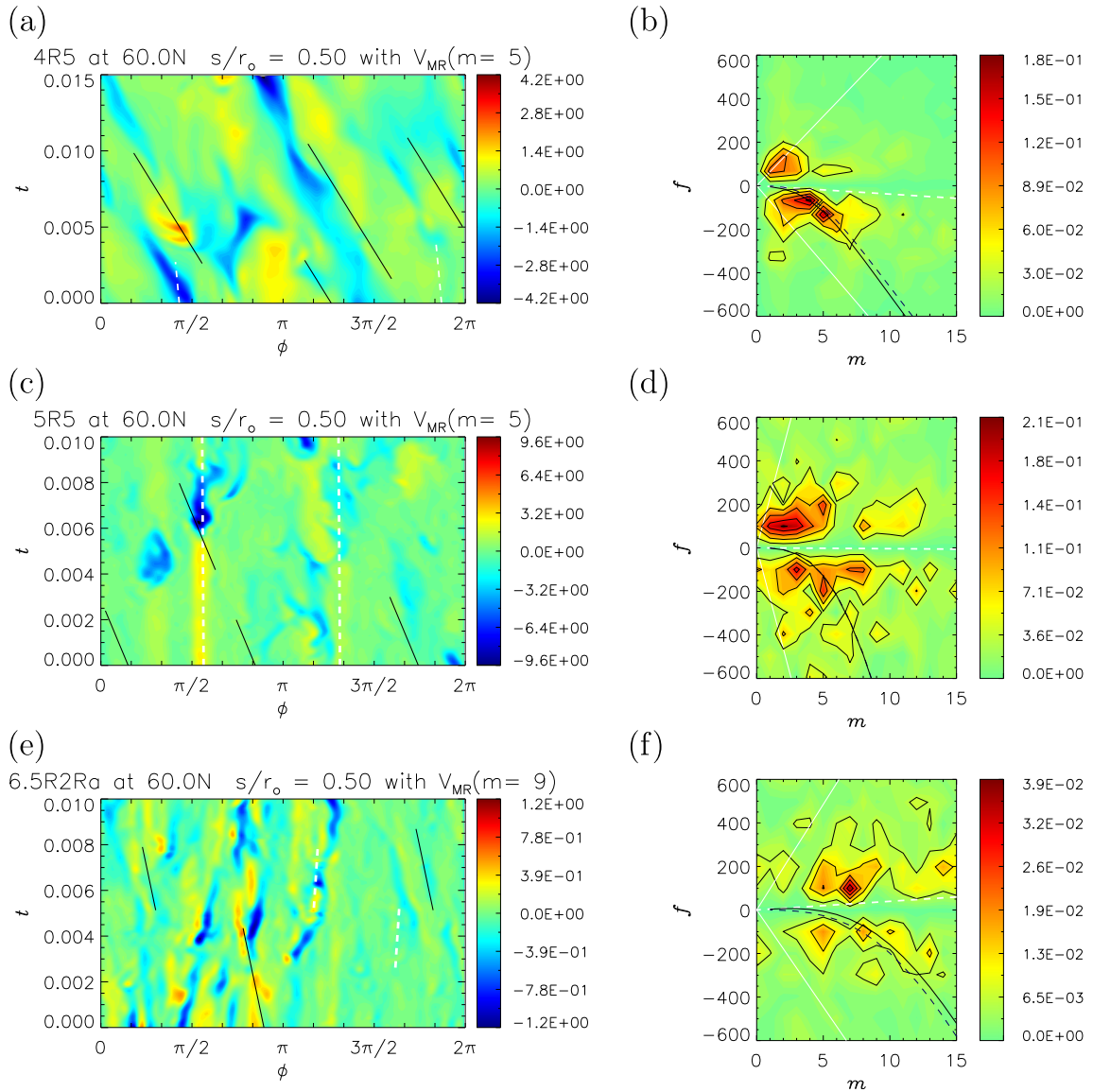
Fig. 13. The residual field B_r at r = r_o at 60^\circ\text{N} for models 4R5 (a-b), 5R5 (c-d), and 6.5R2Ra (e-f). (Left) Azimuth time sections. White dashed and black solid lines represent the speeds \zeta and \zeta + \dot{\omega}_{MR}/m for a given m at s = 0.5r_o , respectively. (Right) Wavenumber - frequency power spectra. White dashed, black dashed, black solid, and white solid curves are the dispersion relations of \omega_{adv}/2\pi , \dot{\omega}_\pm/2\pi , (\omega_{adv} + \dot{\omega}_\pm)/2\pi , and (\omega_{adv} \pm \dot{\omega}_M)/2\pi at the s , respectively.
