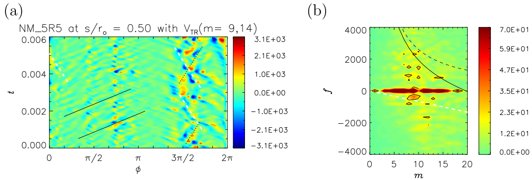
Fig. 8. The radial velocity, \langle u_s \rangle , at radius s = 0.5r_o for the nonmagnetic model NM_5R5 (cf. Fig. 4c-d). White dashed, black solid, and black dotted lines represent the advective speeds ( \zeta ), the total speeds of advection and thermal Rossby wave propagation ( \zeta + \hat{\omega}_{TR}/m ) for m = 9 , and the total speeds for m = 14 , respectively. (Left) Azimuth-time section and (right) wavenumber – frequency power spectrum. In figure (b), white dashed, black dashed, and black solid curves represent the dispersion relations of advection ( \omega_{adv}/2\pi ), waves ( \hat{\omega}_{TM}/2\pi ), and advection plus waves ( (\zeta + \hat{\omega}_{TM})/2\pi ), respectively.
