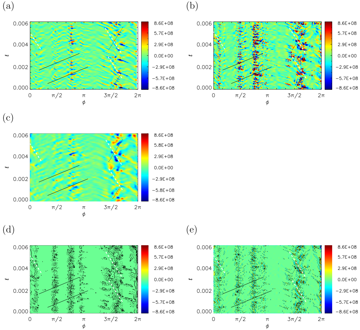
Fig. 9. Terms of the z-averaged vorticity equation, (7) and (8), for the nonmagnetic run NM_5R5 at s = 0.5r_o (cf. Fig. 6). (a) \partial\langle\zeta_z^i\rangle/\partial t , (b) \Xi_R , (c) \Xi_C , (d) \Xi_B , and (e) \Xi_V . Only the fluctuation part excluding the time averages is shown.
