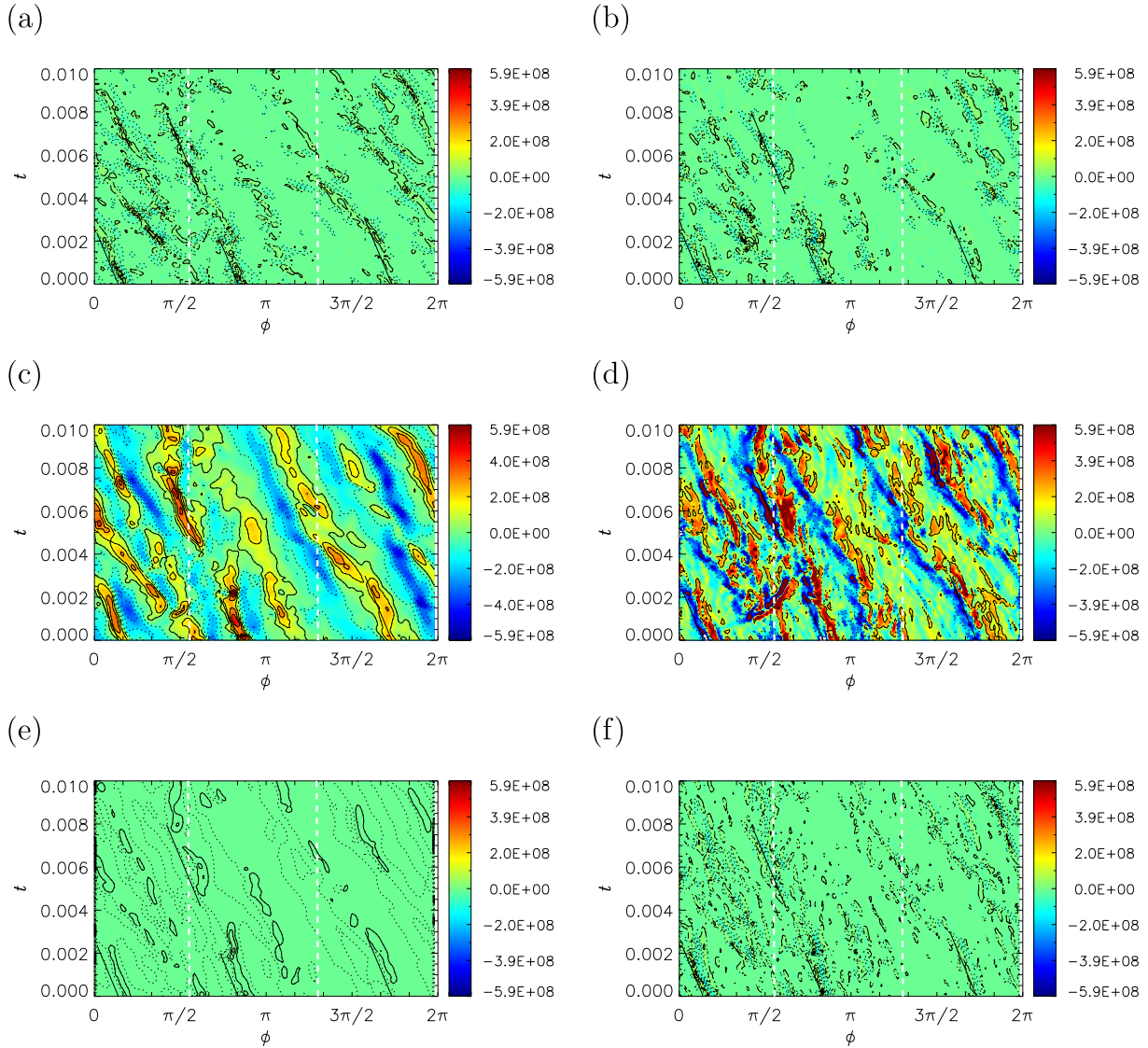
Fig. 6. Terms of the z -averaged vorticity equation, (7) and (8), for model 5R5 at s = 0.5r_0 . (a) \partial(\xi_z^2)/\partial t , (b) \Xi_R , (c) \Xi_C , (d) \Xi_L , (e) \Xi_B , and (f) \Xi_V . Contours for positive (negative) values are indicated by thin solid (dotted) lines. Thick black solid lines represent the total speeds, \zeta + \omega_{MR}/m , for m = 5 . White dashed lines for advection \zeta .
