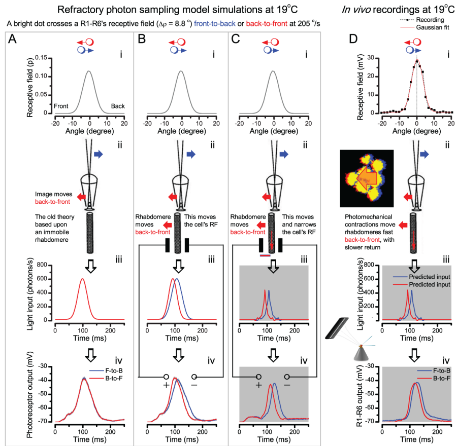
Appendix 8—figure 4. The new hypothesis predicts and the recordings show that R1-R6 output rises and decays earlier to a back-to-front moving bright dot than to a front-to-back moving dot of equal velocity. (A) A classic model with (i) a symmetrical receptive field and (ii) an immobile rhabdome leads to identical (iii) light inputs and virtually identical (iv) photoreceptor outputs (minute differences result from stochastic photon sampling), respectively, for the dots moving in the opposite directions. (B) A model with (ii) a moving rhabdome generates both dynamic (iii) light input and (iv) photoreceptor output, which rise and decay earlier for the back-to-front moving dot (red traces) than the front-to-back moving dot (blue traces). (C) Our full model with rhabdome contraction dynamics that move and narrow its receptive field. This makes the light input and photoreceptor output rise and decay faster than in the other two models, with the back-to-front waveforms leading the front-to-back counterparts. (D) The intracellular responses of a R1-R6 photoreceptor to the given two dot stimuli, as recorded in vivo , show similar dynamics to the full model in (C) with its back-to-front signals (red) leading the front-to-back signals (blue).
