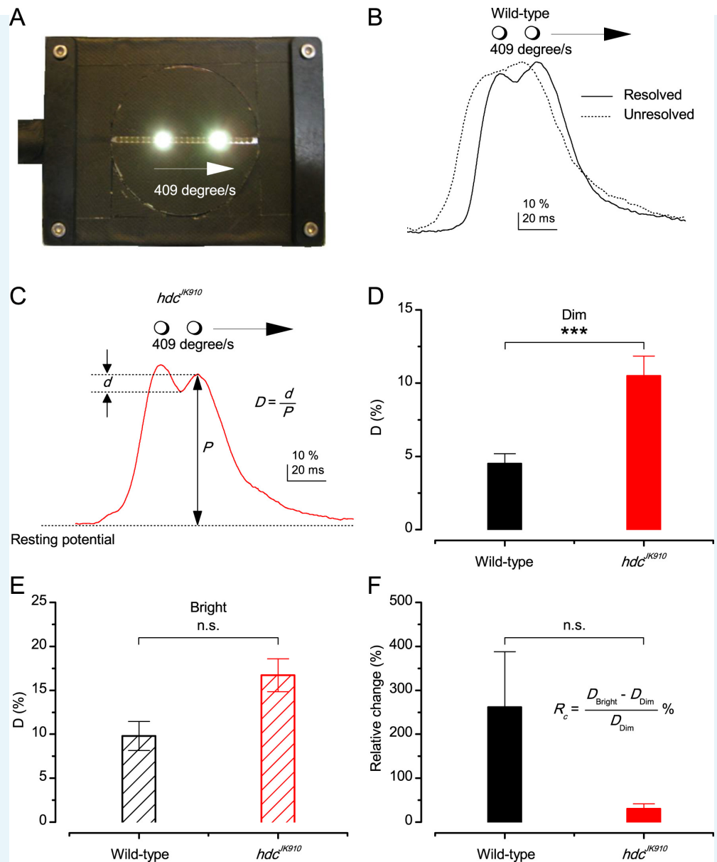
Appendix 6—figure 6. Resolving two moving point-objects. (A) Two light-points (bright dots) moving together were presented in the tested photoreceptor’s receptive field at 19°C. The dots were 6.8° apart and travelled at 409°/s in the front-to-back direction. For clarity, neutral density filters and the LEDs pads used for background illumination are not shown in this picture. (B) In Dim, 12 out of 18 wild-type photoreceptors could resolve them, showing the response waveform depicted by the continuous line, with the larger trailing peak. While six other could not distinguish the two objects; showing the waveform of by the dotted line. In Bright, 5 out of 6 examined wild-type photoreceptors resolved the two dots. (C) Response waveform of hdc JK910 R1-R6s exhibited two distinct peaks, with the leading one was the larger. In Dim, 15 out of 16 tested mutant photoreceptors could resolve the two objects and 14 of them displayed this waveform. In Bright, all of 8 recorded hdc JK910 photoreceptor responses resolved the objects. D-values were calculated from the amplitude of the smaller peak and the dip in between. (D) In Dim, D-values of hdc JK910 R1-R6 responses were significantly larger than their wild-type counterpart. D_{\text{wild-type}} = 4.51 \pm 0.67\% , D_{\text{hdc}} = 10.5 \pm 1.35\% , p = 0.00075 , t-test, n_{\text{wild-type}} = 12 , n_{\text{hdc}} = 15 . (E) In Bright, the difference of D-values of the two photoreceptor groups was statistical insignificant. D_{\text{wild-type}} = 9.81 \pm 1.65\% , D_{\text{hdc}} = 16.71 \pm 1.86\% , p = 0.117 , t-test, n_{\text{wild-type}} = 5 , n_{\text{hdc}} = 8 . (F) .)
