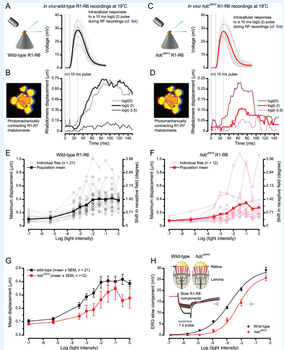
Appendix 7—figure 11. Comparing dark-adapted wild-type and hdc JK910 R1-R6s' photomechanical rhabdomere contractions to their corresponding electrophysiological responses at 19°C. (A) Intracellular voltage responses of dark-adapted wild-type R1-R6s to a 10 ms subsaturating light pulse, delivered at the center of their receptive field. (B) Characteristic non-averaged photomechanical rhabdomere movements (displacement in time) of a typical wild-type fly, as quantified by the cross-correlation analysis ( Appendix 7—figure 4 ) to very dim ( \log(-3.5) ), moderate ( \log(-2) ) and very bright ( \log(0) ) 10 ms light flashes. (C) Intracellular responses of dark-adapted hdc JK910 R1-R6s to a similar stimulus (as in a). (D) hdc JK910 rhabdomere movements to very dim, moderate and very bright 10 ms flashes are characteristically slightly smaller than the corresponding wild-type recordings in (B). (E) The wild-type and (F) hdc JK910 rhabdomere displacements increase with logarithmic light intensity. (G) Mean wild-type rhabdomere movement was larger than that of hdc JK910 over the tested intensity range, with the hdc JK910 photoreceptors' apparent right-shift indicating a 10-fold reduced sensitivity. (H) This right-shift is broadly similar to these photoreceptors' V/LogI characteristics, measured from their ERG slow components ( Dau et al., 2016 ).
