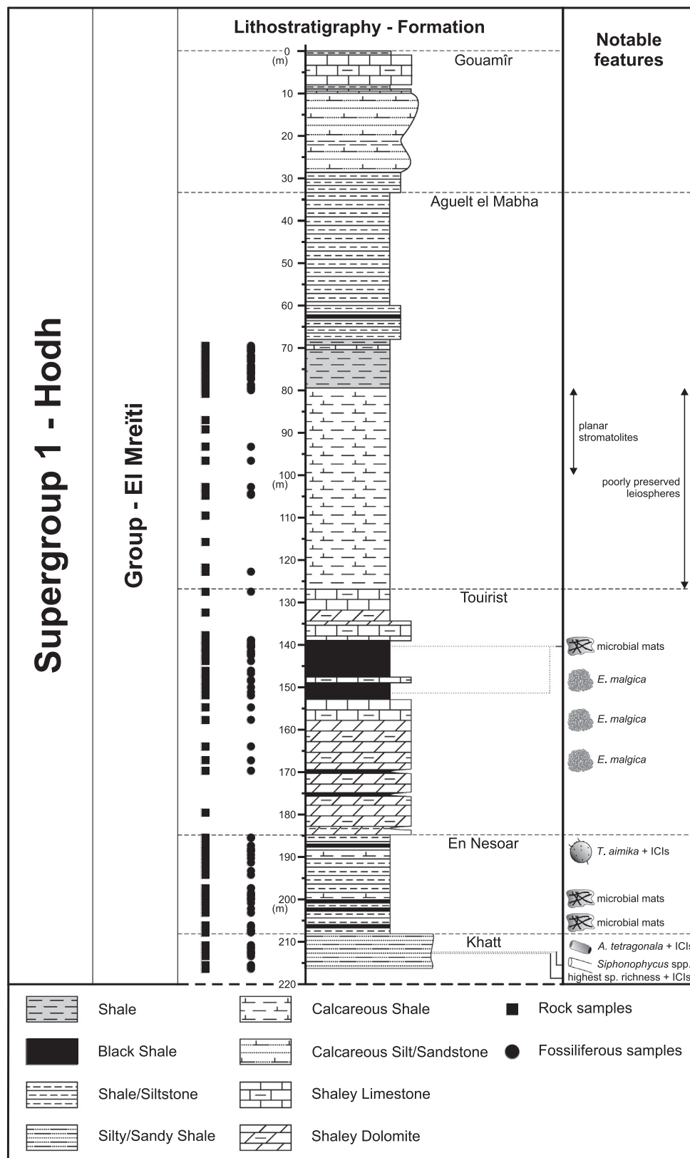
Fig. 3. Generalized lithostratigraphic column of the S2 core – El Mreiti Group (Supergroup 1 – Hodh), Taoudeni Basin, Mauritania modified after Beghin et al. (2017). Right column shows notable features ( \geq 20\% , up to 95%, of relative abundance excepted for Arctacellularia tetragonal and Siphonophycus spp. which are \geq 5\% ; relative abundance of microfossil specimens is calculated without the total number of microbial mats; ubiquitous genera such as Leiosphaeridia and Synsphaeridium are not represented). Quantitative data detailed in Supplementary Table 2. See also Fig. 10. 'ICIs' represents horizons bearing numerous specimens showing inner opaque organic inclusions or intracellular inclusions.
