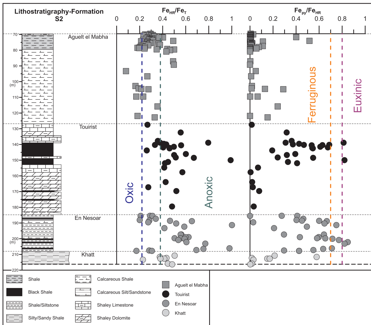
Fig. 4. Generalized lithostratigraphic column of the S2 core – El Mreiti Group (Supergroup 1 – Hodh), Taoudeni Basin, Mauritania modified after Beghin et al. (2017). Iron speciation data of S2: Fe_{HR}/Fe_T and Fe_{Py}/Fe_{HR} .
