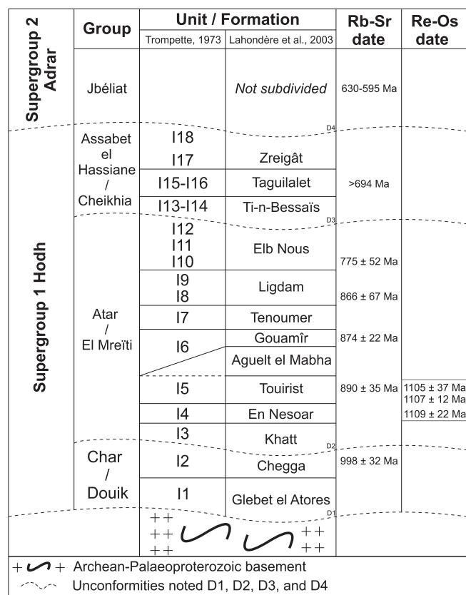
Fig. 2. Stratigraphy of Supergroups 1 (Hodh) and 2 (Adrar) of the Taoudeni Basin. Modified after Beghin et al. (2017) and modified after Rooney et al. (2010). Rb-Sr geochronology data from Clauer (1976, 1981), Clauer et al. (1982), Clauer and Deynoux (1987). Re-Os geochronology datings from Rooney et al. (2010). Stratigraphic nomenclature after Trompette (1973) and Lahond ere et al. (2003). Sinusoidal dashed lines represent unconformities noted D1, D2, D3, and D4 (Lahond ere et al., 2003). Linear dashed lines represent lateral changes.
