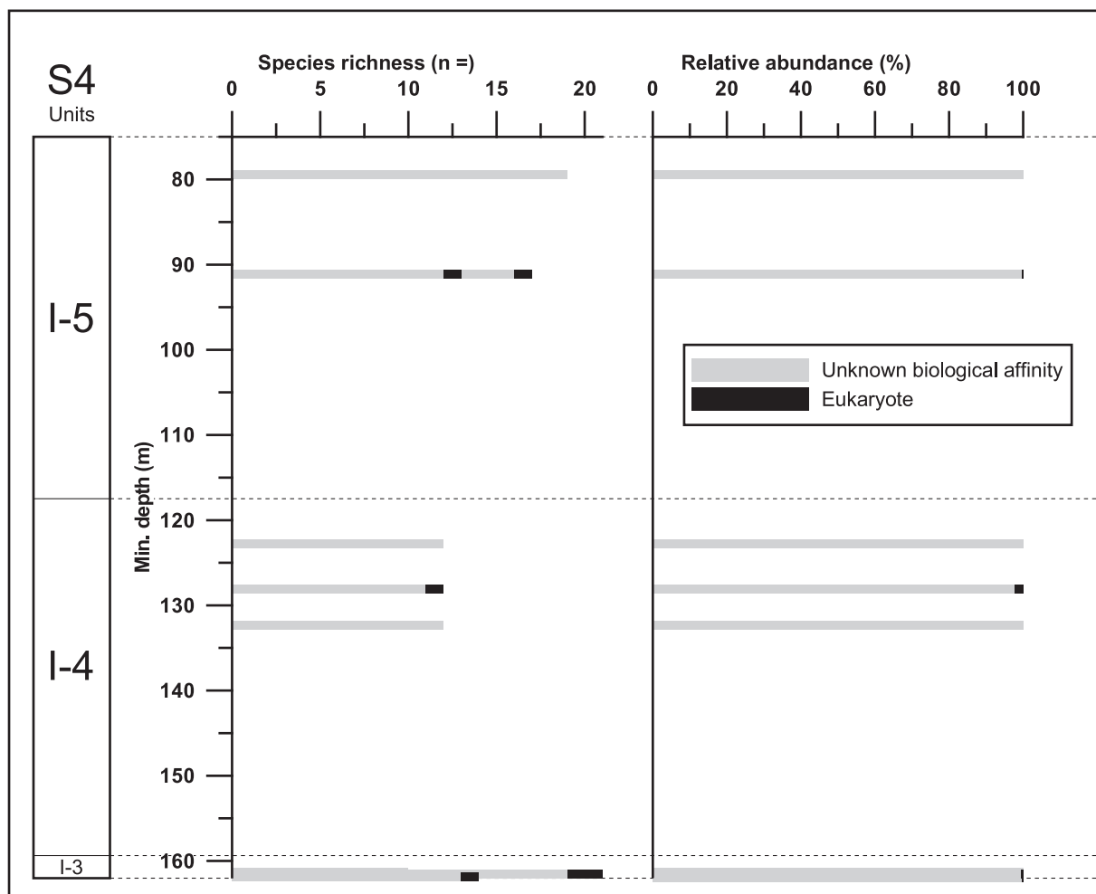
Fig. 7. Quantitative microfossils analysis of S4: species richness ( n = ) and relative abundance (%) of eukaryotes and microfossils of an unknown biological affinity. Atar Group units on the left side.
