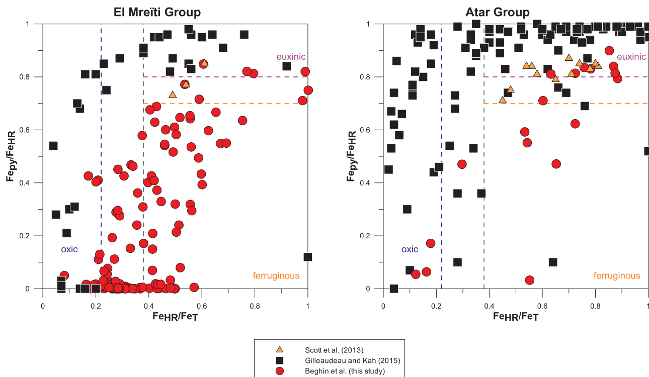
Fig. 8. Iron speciation cross plot ( Fe_{HR}/Fe_T and Fe_{py}/Fe_{HR} ) for all samples from Atar and El Mreïti groups in this study, Scott et al. (2013), and Gilleaudeau and Kah (2015). Fe_{HR}/Fe_T \leq 0.22 = oxic conditions and Fe_{HR}/Fe_T \geq 0.38 = anoxic conditions (vertical dashed lines). Fe_{py}/Fe_{HR} \leq 0.8 or \leq 0.7 = ferruginous conditions and Fe_{py}/Fe_{HR} \geq 0.8 or \geq 0.7 = euxinic conditions (horizontal dashed lines).
