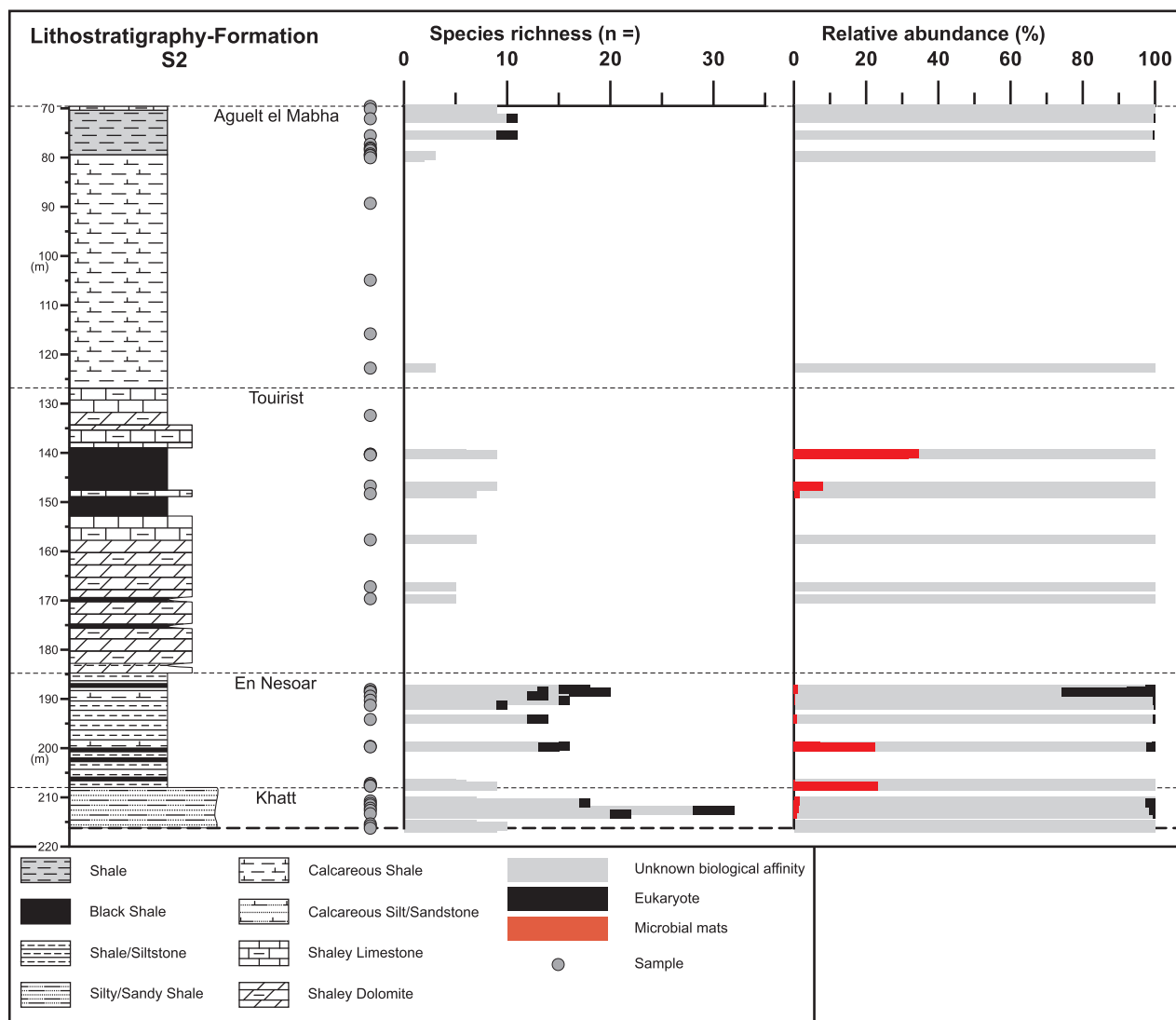
Fig. 6. Generalized lithostratigraphic column of the S2 core – El Mreiti Group (Supergroup 1 – Hodh), Taoudeni Basin, Mauritania modified after Beghin et al. (2017). Quantitative microfossils analysis of S2: species richness (n =) and relative abundance (%) of unambiguous eukaryotes and microfossils of an unknown biological affinity ( incertae sedis ). Relative abundance of microfossil specimens is calculated without the total number of microbial mats. Microbial mats are not counted in the total species richness. Relative abundance of microbial mats is calculated separately (see Supplementary Table 2).
