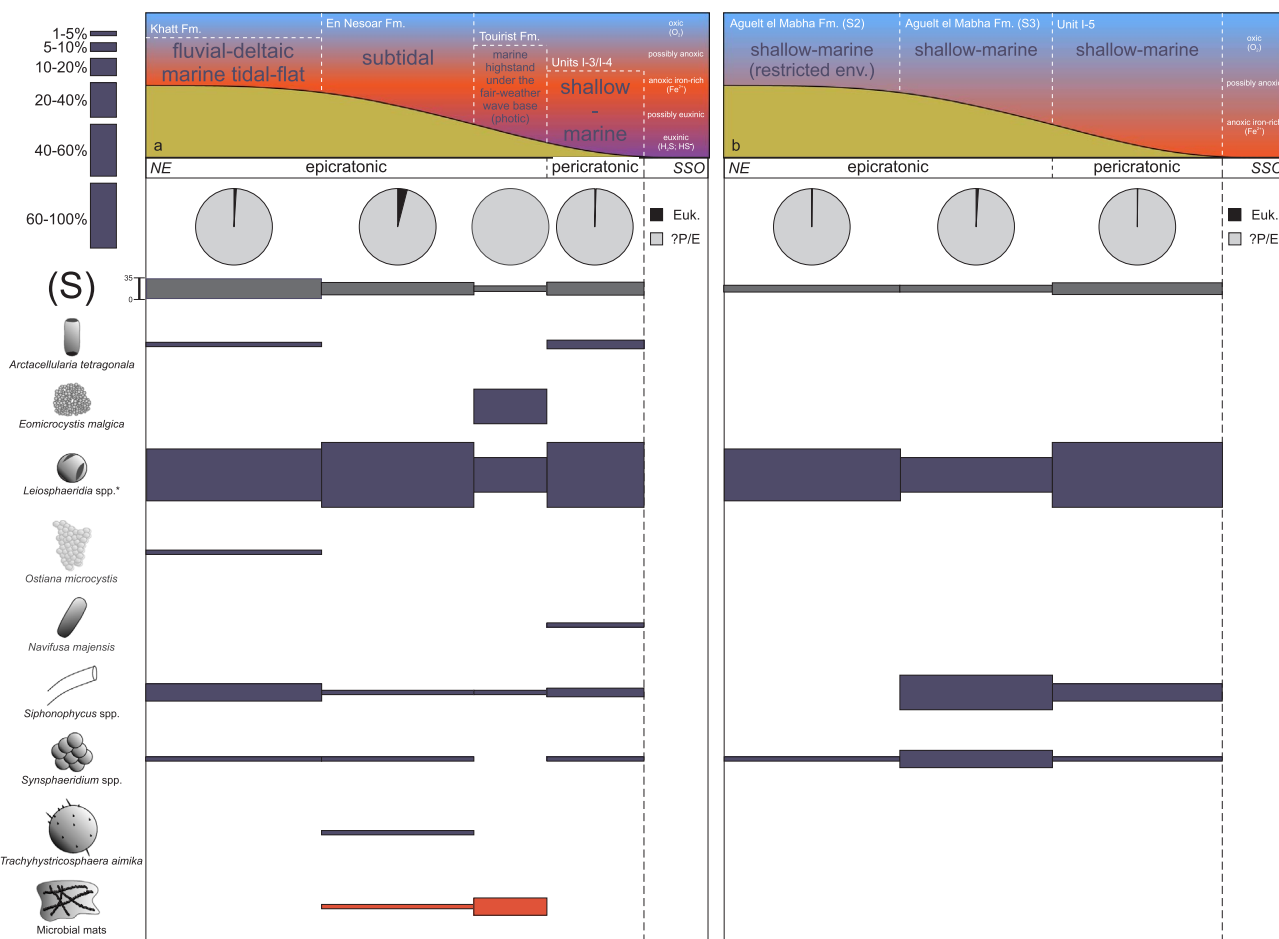
Fig. 10. Palaeoecological distribution of the Atar/El Mreiti Group dominant species and features. (a) Marine transgression and (b) marine regression. (S) is species richness. Blue line width is proportional to the species relative abundance (%) calculated for a defined palaeoenvironment (dashed white line): total number of specimens counted for one species/total number of specimens counted within one defined palaeoenvironment). Leiosphaeridia spp. * means all species of the genus Leiosphaeridia except L. kulgunica and poorly preserved leiospheres. Spumosina rubiginosa and Polytrichoides lineatus are not represented. Relative abundance of microfossil specimens is calculated without the total number of microbial mats. (For interpretation of the references to colour in this figure legend, the reader is referred to the web version of this article.)
