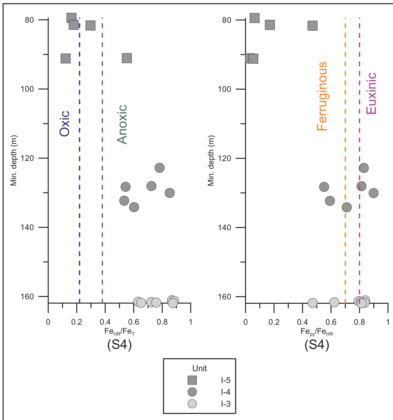
Fig. 5. Iron speciation data of S4: Fe_{HR}/Fe_T and Fe_{Py}/Fe_{HR} .
