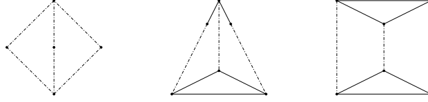
Fig. 1. Theta, pyramid and prism. (A full line represents an edge, and a dashed line represents a path of edge-length at least one.)
