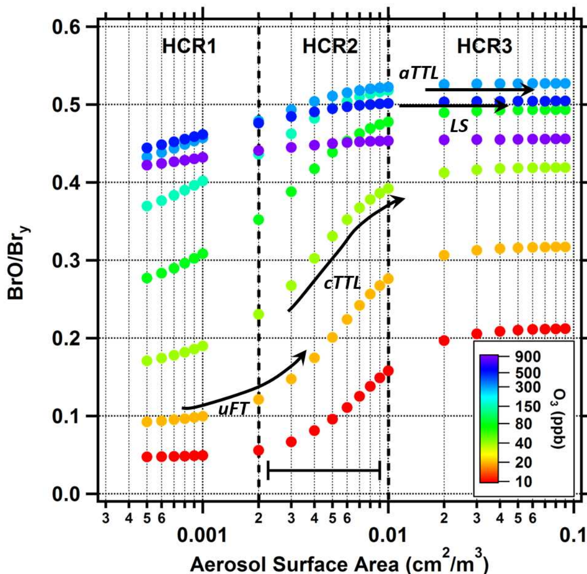
5 Figure 5: Sensitivity of the BrO/Br y ratio surface area (to SA) and O 3 concentration. Conditions are representative of the upper troposphere. (dashed vertical lines) mark the heterogeneous chemical regimes (HCR, see Sect. 2.3.1). The horizontal bar at the bottom marks a factor of four in SA along the logarithmic abscissa (i.e., the difference between case 0 and case 1). Arrows mark the corresponding sensitivity of the BrO/Br y ratio in the upper FT (uFT), convective TTL (cTTL), aged TTL (aTTL), and LS. The largest sensitivity is observed in the upper FT and convective TTL, while the aged TTL and LS are insensitive.
