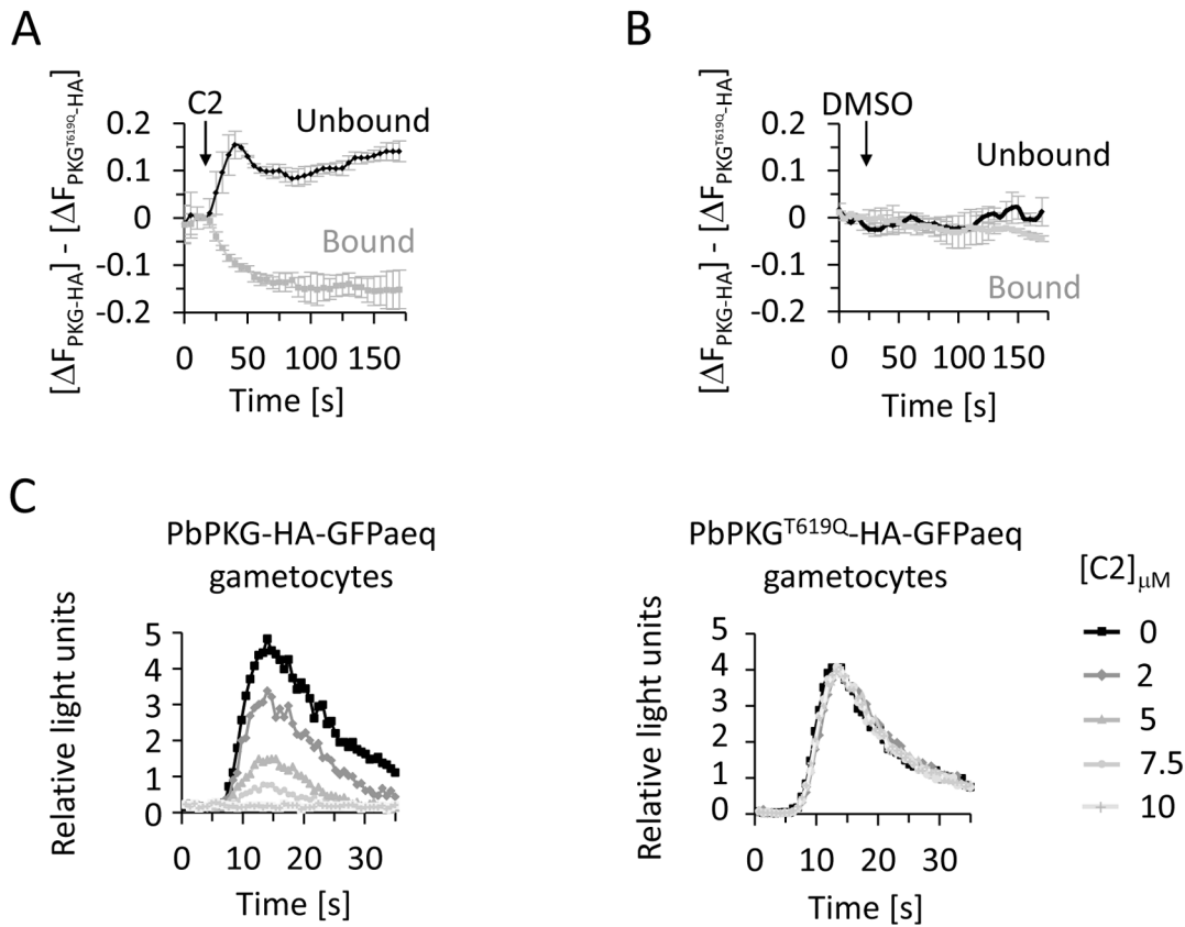
Figure 5. PKG controls cytosolic Ca^{2+} levels in ookinete and upon gametocyte activation in P. berghei . (A and B) Determination of relative cytosolic Ca^{2+} levels in purified ookinetes expressing PKG-HA or PKG T619Q -HA using pericam, a dual excitation Ca^{2+} reporter. We added 0.5 \mu M C2 treatment (A) or DMSO treatment (B) at t = 20 s. Fluorescence was normalised as follows: \Delta F = (F_n - F_{20})/F_{20} , in which F_n is the fluorescence at t = n s; F_{20} is the reference time before addition of C2 or DMSO, and was normalised to the baseline provided by the C2-resistant parasites expressing PKG T619Q -HA. Error bars show standard errors from three independent replicates each using 10 ookinetes per condition. See Figure S6A and Figure S6B for a validation of the pericam reporter in P. berghei . (C) Luminescence responses of gametocytes expressing GFP-aequorin to different concentrations of C2. Gametocytes were stimulated with 50 \mu M XA at t = 0 s. Data are representative of at least four independent experiments. doi:10.1371/journal.pbio.1001806.g005
