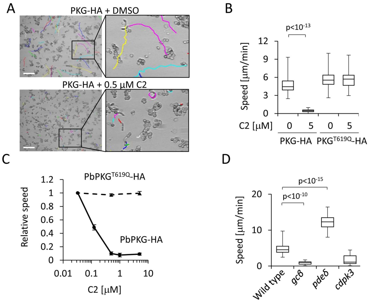
Figure 1. Role of PKG in regulating ookinete gliding. (A) Gliding traces of ookinetes in matrigel recorded for 20 min from a representative field of view. Scale bar, 50 μm. The coloured tracks were created by superimposing individual images from a time series, each marking the tip of each ookinete. (B) Effect of C2 on the gliding speed of ookinetes. (C) Average gliding speed of ookinetes at increasing concentrations of C2. Error bars show standard deviations of 20 ookinetes from each of two independent biological replicates. (D) Gliding speeds of mutant ookinetes. The range of whisker plots in (B) and (D) indicates the 2.5 and 97.5 percentiles, the box includes 50% of all values, and the horizontal line shows median values obtained for 20 ookinetes from each of two independent biological replicates. Statistical analyses in (B) and (D) were carried out using a two-tailed t test. doi:10.1371/journal.pbio.1001806.g001
