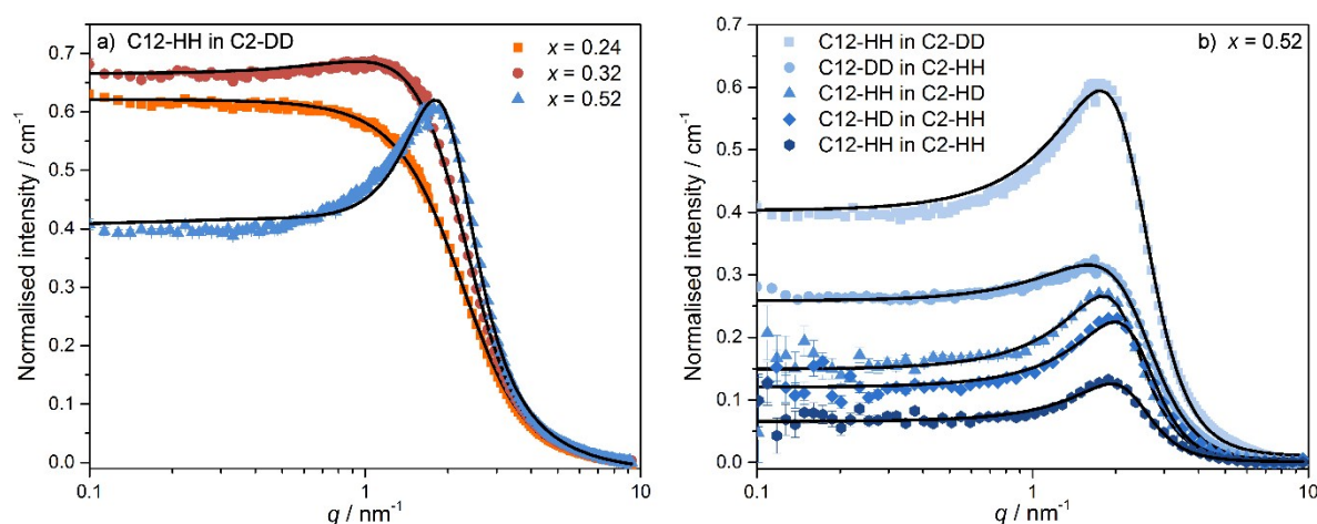
Figure 5: SANS data for [C_{12}mim-d_{11}]_{1-x}[C_{12}mim]_x[Tf_2N] : Panel a) where 0.24 \leq x \leq 0.52 and panel b) all contrasts for x = 0.52 . Fits to the Teubner-Strey model are shown as black lines.
