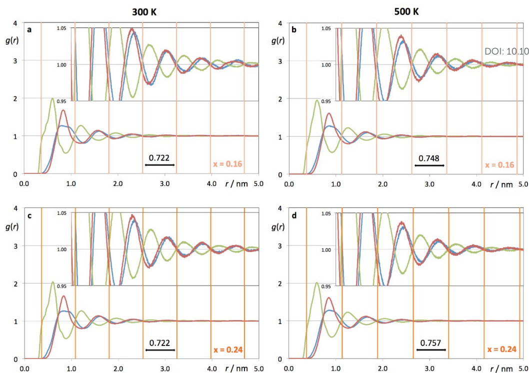
Figure 14: Pair radial distribution functions, g(r) , for x = 0.16 and 0.24 at 300 K and 500 K. Green curves: cation-anion g(r) s (imidazolium ring centroid to nitrogen atom, CM-NBT); red curves: anion-anion g(r) s (NBT-NBT); blue curves: cation-cation g(r) s (CM-CM). The vertical orange lines and numerals indicate the characteristic wavelength of the dampened periodical functions.
