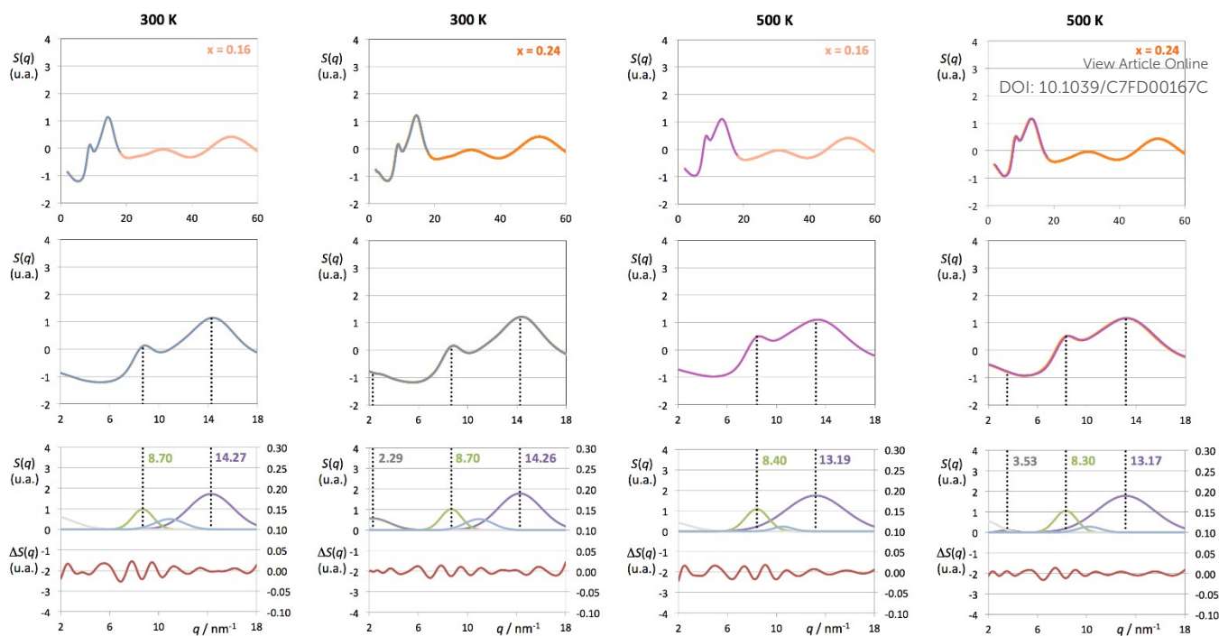
Figure 13: Structure factor functions, S(q) , for [\text{C}_2\text{mim}]_{1-x}[\text{C}_{12}\text{mim}]_x[\text{TF}_2\text{N}] mixtures, where x = 0.16 and 0.24 at 300 K and 500 K. The top row is the S(q) function in the full q -value range studied ( 2 < q/\text{nm}^{-1} < 60 ), where the grey parts of the data are the low- q regions focused on in the discussion; in the second row the focus is on the low- q values and the bottom row is the deconvolution of the low- q peaks and the fitting deviation.
