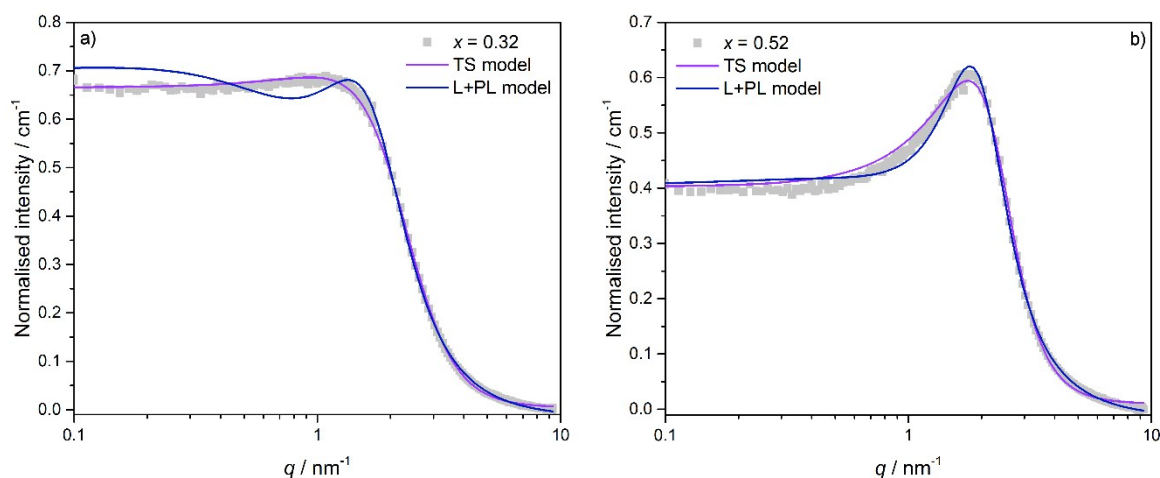
Figure 6: SANS data for [C_2mim-d_{11}]_{1-x}[C_{12}mim]_x[Tf_2N] (fits to other contrasts are similar): Panel a) x = 0.32 and panel b) x = 0.52 . Fits to the Teubner-Strey (TS model) and Lorentz + Peak Lorentz (L+PL model) are shown in purple and blue respectively.
