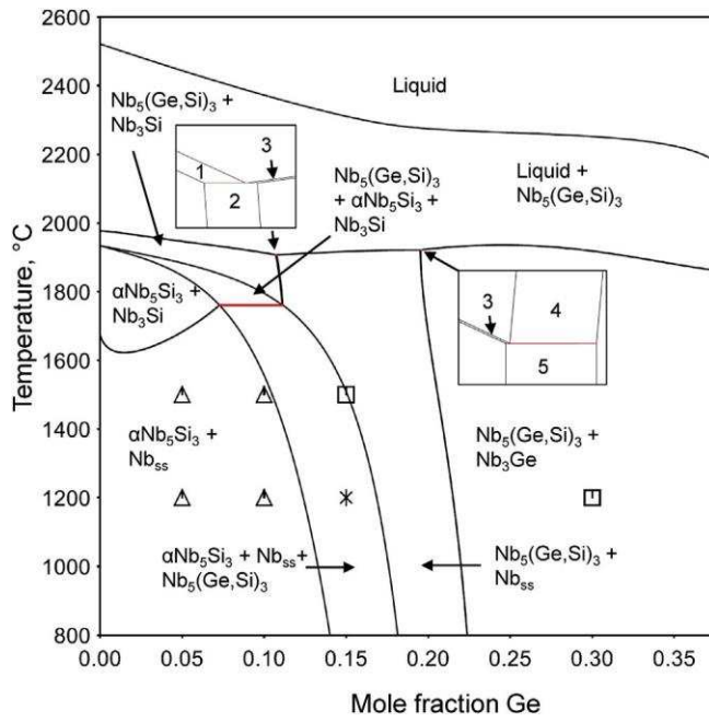
Fig. 12. Isoleth section at x(\text{Nb}) = 0.625 with experimental data from current work. Key: triangle - \alpha\text{Nb}_5\text{Si}_3 , star - \alpha\text{Nb}_5\text{Si}_3 + \beta\text{Nb}_5\text{Si}_3 , square - \beta\text{Nb}_5\text{Si}_3 . Insets show thin phase regions. Numbers refer to phase regions: 1: \text{L} + \text{Nb}_3\text{Si} + \text{Nb}_5(\text{Ge,Si})_3 , 2: \text{Nb}_{ss} + \text{Nb}_3\text{Si} + \text{Nb}_5(\text{Ge,Si})_3 , 3: \text{L} + \text{Nb}_{ss} + \text{Nb}_5(\text{Ge,Si})_3 , 4: \text{L} + \text{Nb}_3\text{Ge} + \text{Nb}_5(\text{Ge,Si})_3 , 5: \text{Nb}_{ss} + \text{Nb}_3\text{Ge} + \text{Nb}_5(\text{Ge,Si})_3
