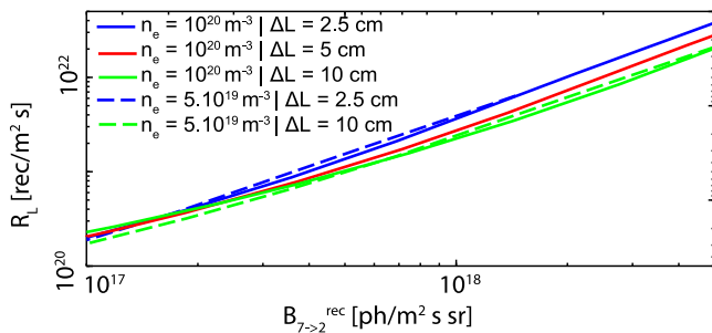
Fig. 3. Modelled relation between the R_L and B_{7 \rightarrow 2}^{rec} for a range of different n_e and \Delta L .
