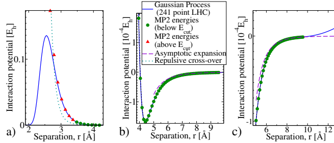
FIG. 3. \text{CO}_2\text{-Ne} Molpro calculations and the GP model, at \cos\theta = 1 (linear geometry), in the repulsive (a), attractive (b) and long-range (c) regions. The long-range asymptotic expansion is E = -(0.570 + 0.182 \cos^2\theta)r^{-6} - (1.704 + 7.266 \cos^2\theta + 1.785 \cos^4\theta)r^{-8} .
