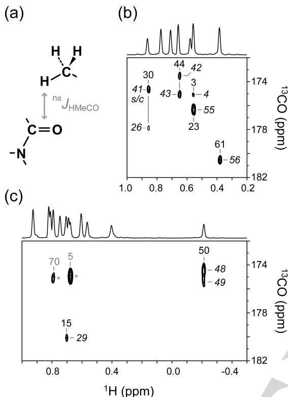
Figure 3. Detection of {}^n J_{\text{HMeCO}} couplings in proteins. (a) Schematic showing the through-space {}^n J_{\text{HMeCO}} coupling detected between methyl protons and backbone carbonyl carbon; (b) carbonyl region of a 2D {}^1\text{H} - {}^{13}\text{C} HMQC spectrum recorded of [ U - {}^2\text{H} , {}^{13}\text{C} , {}^{15}\text{N} ], Ile- [\delta_1 - {}^{12}\text{C}^1\text{H}_3 ]-labeled ubiquitin. “s/c” indicates side chain carbonyl acceptor (c) carbonyl region of a 2D {}^1\text{H} - {}^{13}\text{C} HMQC spectrum recorded of [ U - {}^2\text{H} , {}^{13}\text{C} , {}^{15}\text{N} ], Leu/Val- [\delta_1 - {}^{12}\text{C}^1\text{H}_3 ]-proS-labeled ubiquitin. Asterisks indicate cross peaks arising from through-bond {}^5 J couplings. Above each data set is the 1D projection of a 2D ( {}^1\text{H} , {}^{13}\text{C} ) SOFAST-HMQC spectrum of a [ {}^{13}\text{C}^1\text{H}_3 ]-methyl labeled ubiquitin sample.
