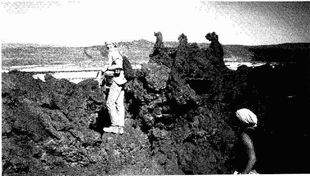
Figure 5.5 Lava flow in the Manda Volcanic system showing the typical height and jaggedness of a young feature. These pose a barrier to movement but are not insurmountable by bipeds.
