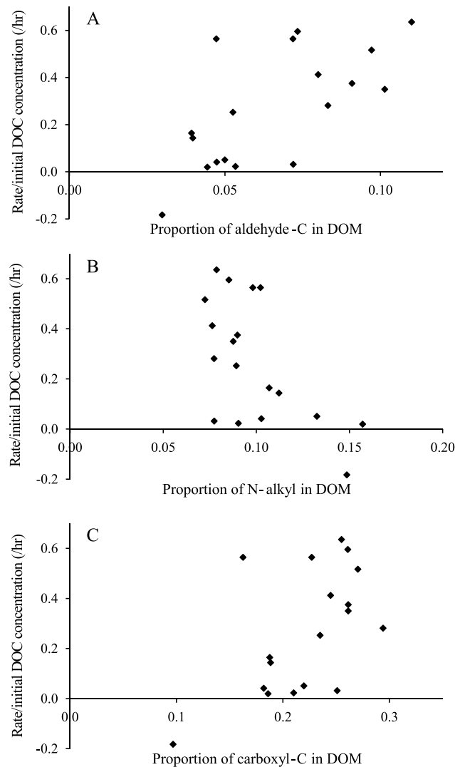
Figure 4. The comparison of the specific initial rate (per hour) to the proportion of (a) aldehyde-C, (b) N-alkyl C, and (c) carboxyl-C.
