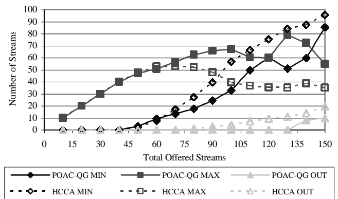
Fig. 11. The number of the traffic streams assigned the minimum quality level or the maximum quality level or they were rejected versus the number of the total offered traffic streams
