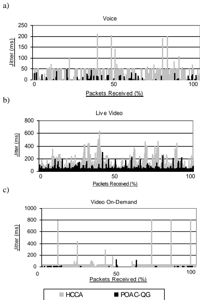
Fig. 7. Packet jitter measurements concerning a) voice, b) live video, and c) video on demand traffic
