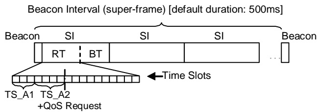
Fig. 2. The POAC-QG superframe
