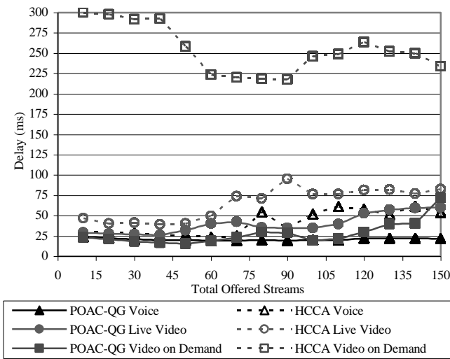
Fig. 9. Average packet delay versus the number of total offered traffic streams
