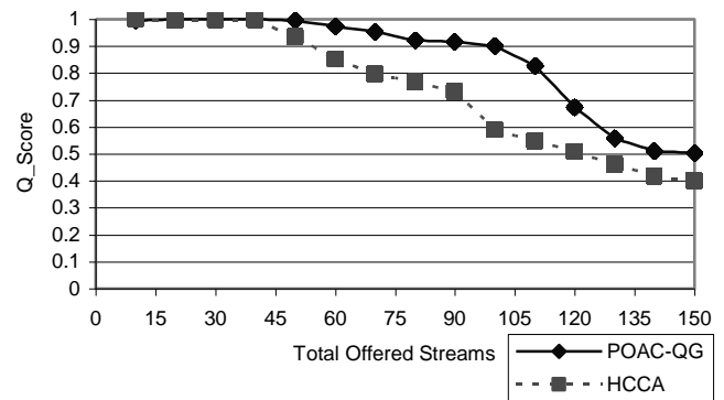
Fig. 10. Q_Score versus the number of the total offered traffic streams
