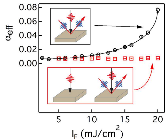
FIG. 4. Pump irradiation fluence ( I_F ) dependence of effective damping constants extracted at the field of 4900 \text{ Oe} . The black circles represent the effective damping constants under different pump fluences; whereas, the effective damping constants represented by the red squares were obtained at a fixed pump fluence of 5 \text{ mJ/cm}^2 , before which the sample was exposed under the indicated illuminations of the laser pulse. The measurement configurations for black circles and red squares are illustrated in the upside and downside of insets, respectively. The solid line is a guide to eyes.
