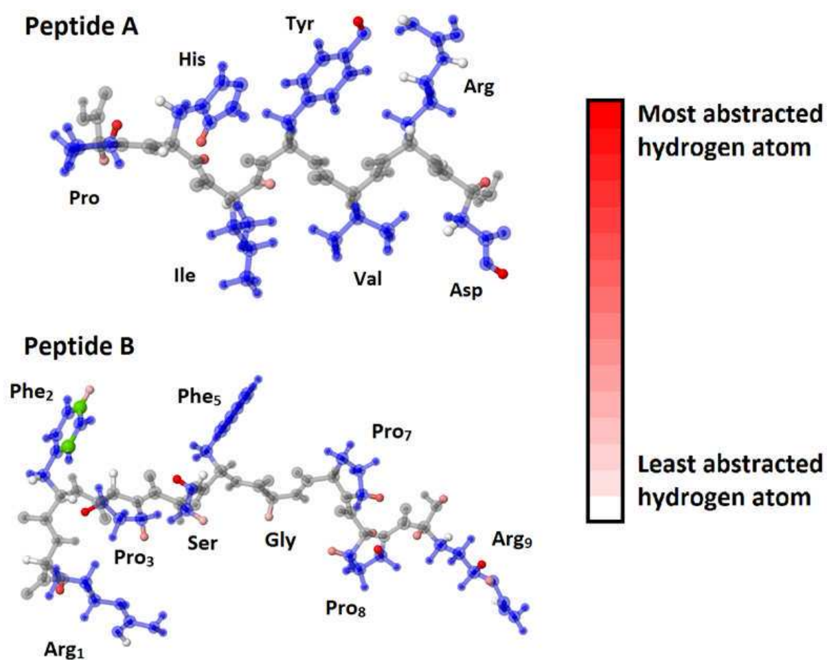
Figure 4. Snapshot of the 3D representation of the oxidation sites in both peptides. The H-atoms most prone to H-abstraction reactions are depicted as red solid spheres, using a scale ranging from pale to intense red, representing the range from least abstracted to most abstracted H-atoms. The green spheres indicate the
