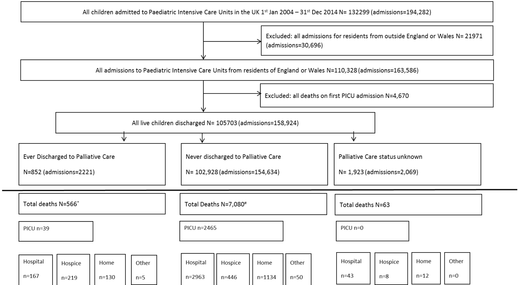
Figure 1 Study Flowchart
