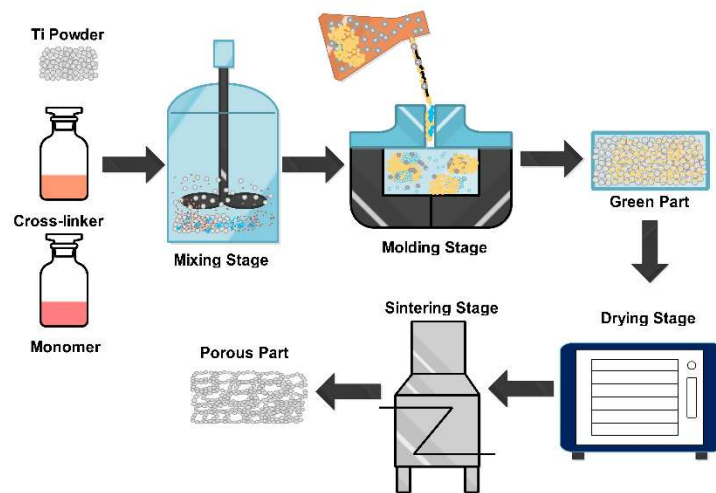
Fig. 4 – A schematic diagram of the gel casting process.
