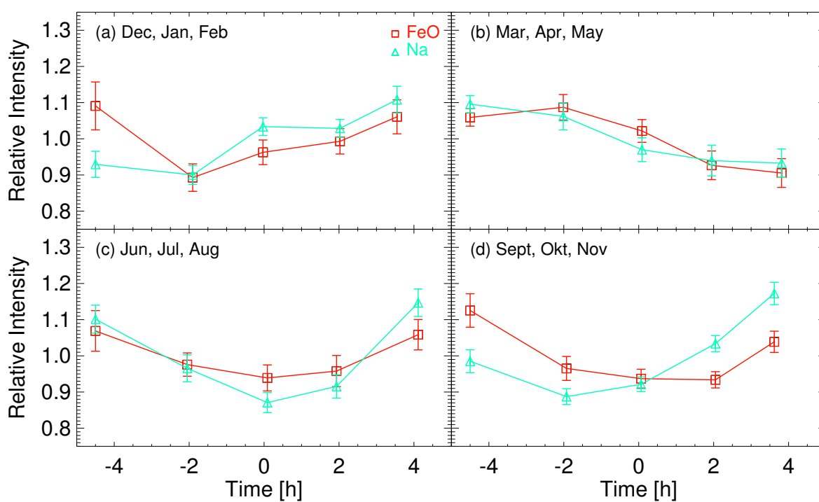
Figure 4. Diurnal variability with respect to season. The colours indicate the emitter: FeO (red squares), Na (cyan triangles). The symbols are placed at the mean time of all the measurements in each bin with respect to midnight. The ordinate shows the intensities relative to the nocturnal average.
