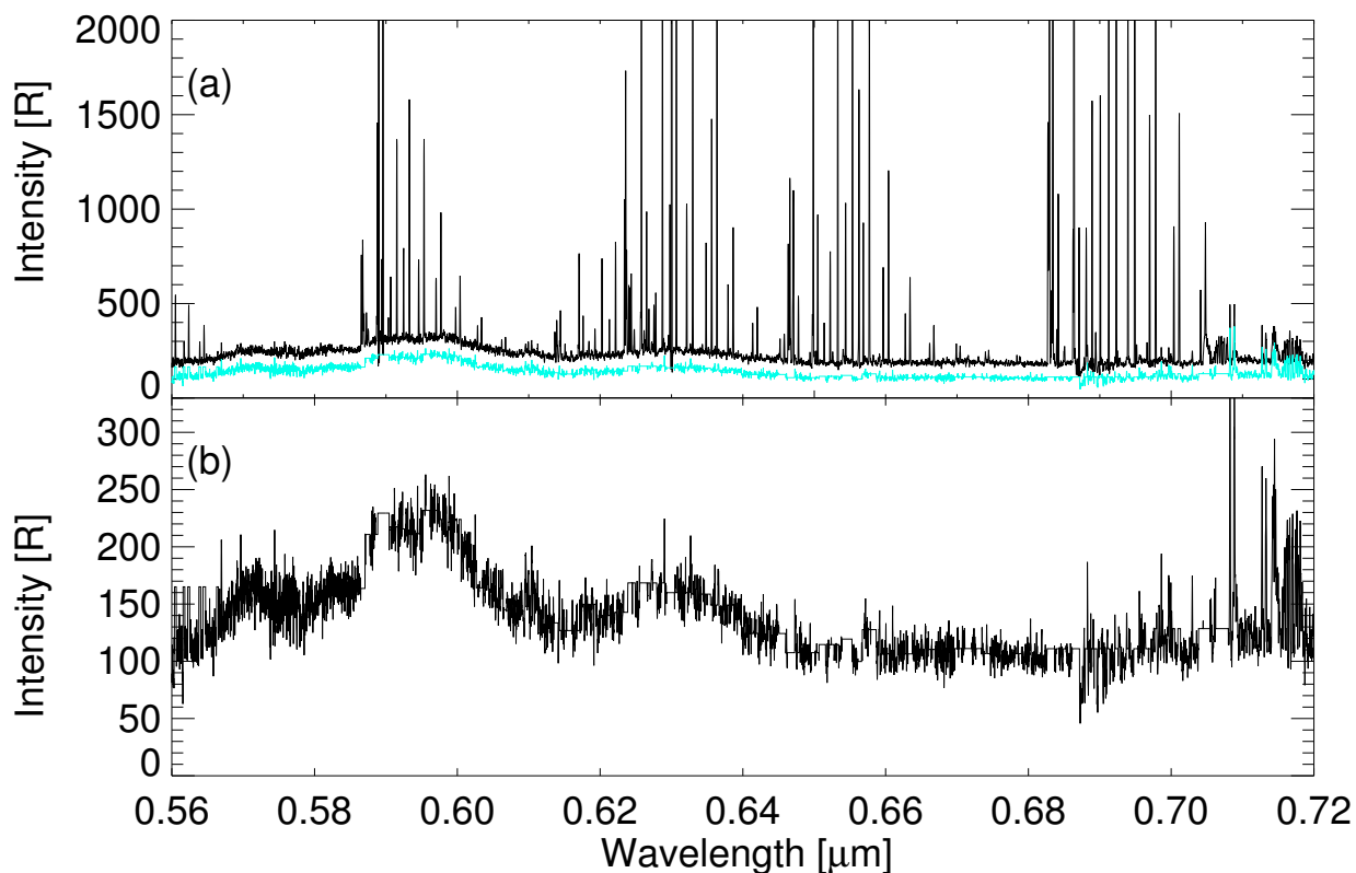
Figure 2. Example of a FeO spectrum. Panel (a) displays a raw night-sky spectrum with all its emissions. The FeO continuum, with possible contamination by NiO and NO+O, is overplotted in cyan. Panel (b) shows the same spectrum after removal of all airglow emission lines, zodiacal light, scattered star- and moon light. The spectrum has an exposure time of 3 600 sec and a resolving power of 7 450. The ordinate shows the emission intensity in Rayleighs ( 1\text{R} = 10^6 \text{ photons cm}^{-2} \text{ s}^{-1} ) while the abscissa shows the FeO emission regime in \mu\text{m} .
