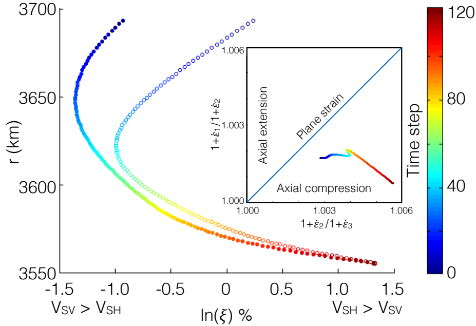
Fig. 7. Predicted seismic anisotropy along a pathline inside the post-perovskite stability field ending at 30^{\circ}\text{N} 90^{\circ}\text{W} and 75 km above the CMB. Filled circles represent the anisotropy when texture is inherited during the bridgmanite to post-perovskite phase transition and open circles represent the case when the initial texture is represented by 500 post-perovskite crystals drawn from a uniform random distribution (the slight positive anisotropy in this case is due to the limited number of grains included in the calculation). The colours represent the time step along the pathline (each representing 25 kyear) from the point where the pathline first crosses the phase boundary (blue, 215 km above the CMB at approximately 26^{\circ}\text{N} and 84^{\circ}\text{W} ) to the point 122 time steps later where the particle arrives 75 km above the CMB. The inset graph shows the evolution of the strain rate tensor along the same pathline. Points represent ratios of the eigenvalues of the strain rate tensor such that plane strain plots along the diagonal with axial compression and extension plotting towards the axes. Time step is represented using the same colours as in the main figure. For all points the vorticity number is less than 1 (representing simple shear) and it increases from \sim 0.5 at the start of the pathline to \sim 0.7 as the pathline approaches the CMB.
