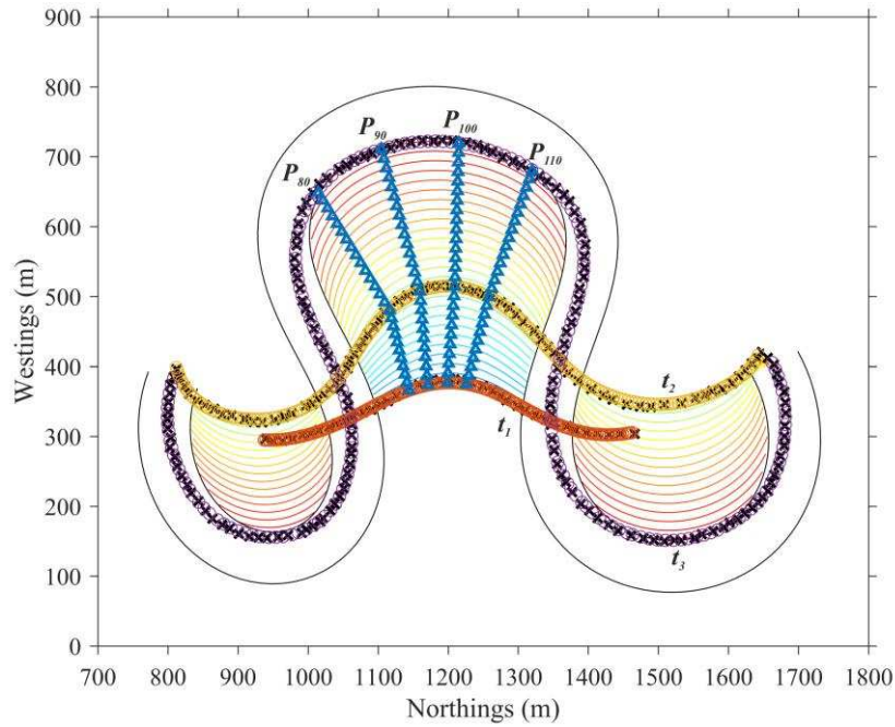
Fig. 4. An example of modelling point bar evolution in plan view. Black crosses denote input data at three key times ( n_{t_1} = 39 , n_{t_2} = 73 , and n_{t_3} = 154 ). For each of these times, these data are then smoothed with a Savitzky-Golay filter that uses a polynomial order of 3 and a frame length of 21. Smoothed data are then extrapolated to control points (200 in this case) at each time, shown in red circles at t_1 , yellow circles at t_2 , and purple circles at t_3 , respectively. Bar positions between these key times are interpolated linearly. Trajectories of four representative ( P_{80} , P_{90} , P_{100} , and P_{110} ) points are shown in blue triangles.
