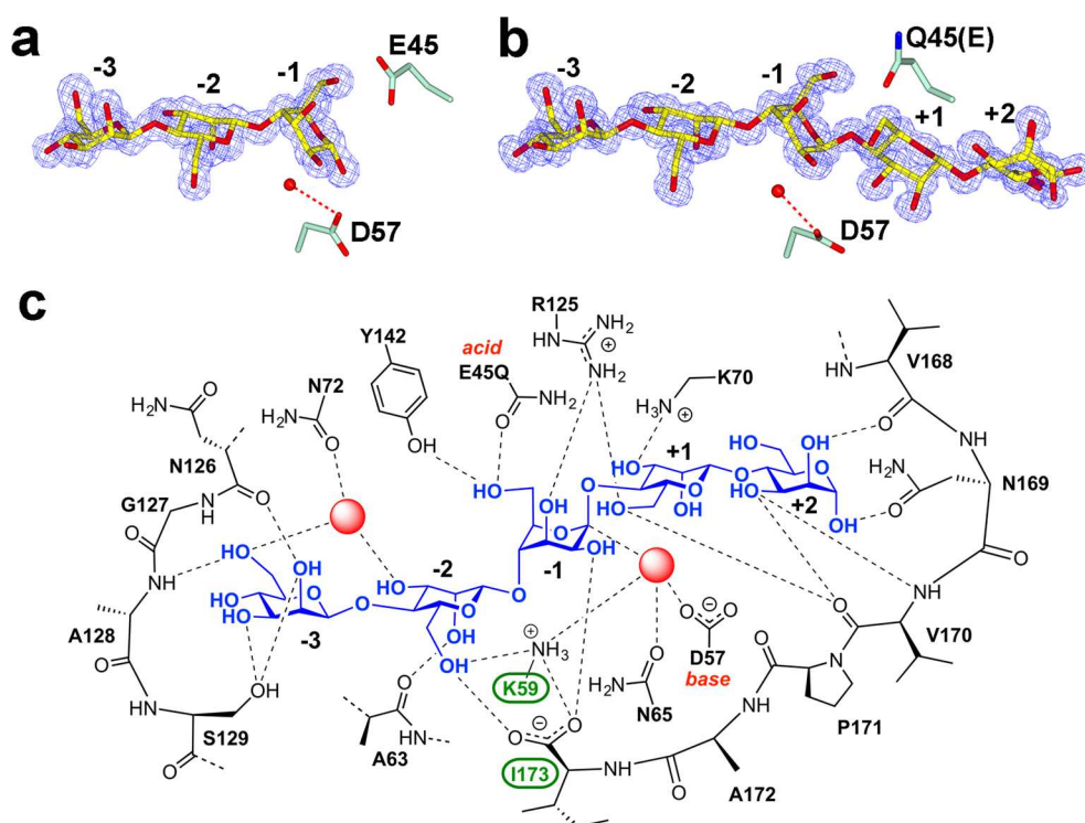
Figure 4. Complexes of (a) wild-type SsGH134 with M3 and (b) E45Q variant with M5 showing the proposed general acid (E45/Q45) suitably positioned near the fissile glycosidic bond, and on the opposing side the proposed general base D57, coordinating the nucleophilic water molecule. Electron density meshes are \sigma A-weighted 2F_o - F_c contoured at 1\sigma (0.58 and 0.47 electrons per \text{\AA}^3 , respectively), assembled using CCP4mg. 33 (c) Cartoon showing major protein substrate interactions for the SsGH134–mannopentaose complex. Interactions are shown for the model of the SsGH134 bound to the \alpha -anomer of \beta -1,4-mannopentaose. The red spheres denote water molecules.
