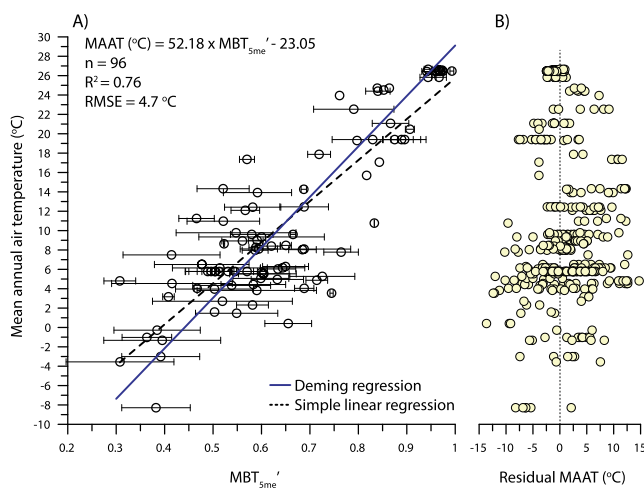
Fig. 10. Average MBT_{5me}^t for each peat versus MAAT (black circles). The solid blue line represents the Deming regression, whereas dashed lines reflect the simple linear regression. Horizontal error bars represent 1\sigma and are based on the analysis of multiple horizons from the same peat. Also shown is the residual MAAT of all analyzed peat samples (yellow circles) obtained by subtracting the estimated MAAT using the MBT_{5me}^t Deming calibration from the observed MAAT. (For interpretation of the references to color in this figure legend, the reader is referred to the web version of this article).
