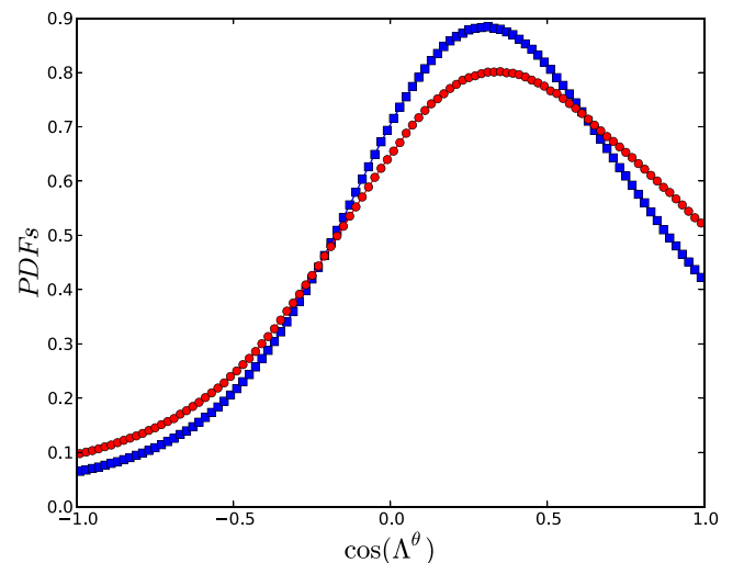
FIG. 15. PDFs of the cosine of the angle between \tau_i^\theta and \partial_i \tilde{\theta} , \Lambda^\theta . Blue squares: MTLM fields. Red circles: DNS fields.
