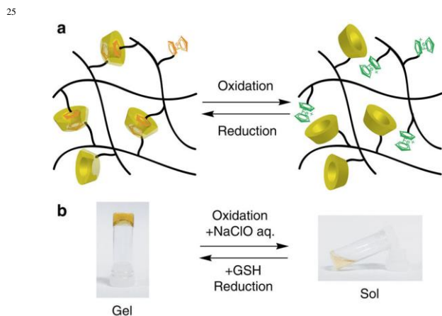
Fig. 21 (a) Schematic illustration of sol-gel transition on ferrocenyl-cyclodextrin materials. (b) Sol-gel transition experiment using chemical oxidant and reductant. Adding NaClO aq. to the pAA- \beta CD/pAA-Fc hydrogel gives a phase transition into the sol state, and continuous addition of glutathione (GSH) to the sol yields a hydrogel again (reproduced with permission from ref. 47).
