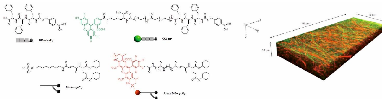
Fig. 4 Structures of self-assembling systems investigated by Hamachi and co-workers, with the Three-dimensional CLSM image of the four-component mixture (BPmoc-F 3 /Phos-cycC 6 /OG-BP/Alexa546-cycC 6 ). The three-dimensional CLSM image is constructed from z-stacked x–y slice images (Supplementary Movie 1). The scale of the z axis is compressed to one-third for clarity. Conditions: [BPmoc-F 3 ] = 0.10 wt% (1.6 mM), [Phos-cycC 6 ] = 0.10 wt% (1.6 mM), [OG-BP] = 0.0005 wt% (3.2 μM), [Alexa546-cycC 6 ] = 0.0005 wt% (3.4 μM) in 100 mM MES buffer (pH 7.0).
