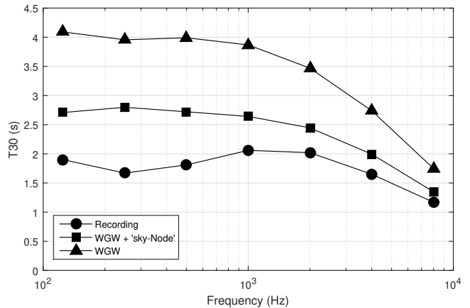
Fig. 19. Octave band reverberation time results for the IR measurement/recording obtained from the urban courtyard and from two WGW simulations made using the same 5-node layout with one also including an absorptive ‘sky-node’.
