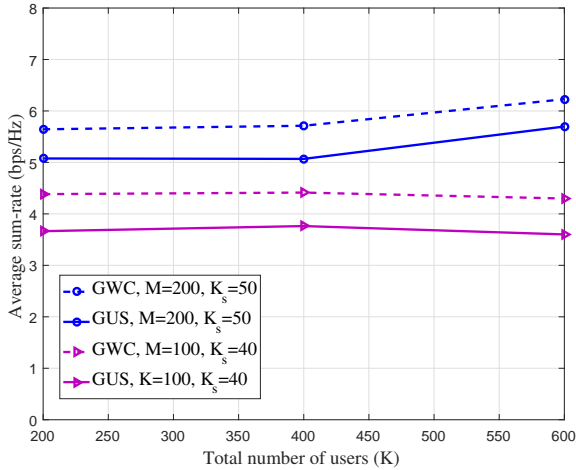
Fig. 4. The average sum-rate vs. total number of users for different values of M = 200 , M = 100 , K_s = 50 , K_s = 40 , R = 600m and R = 1000m .
