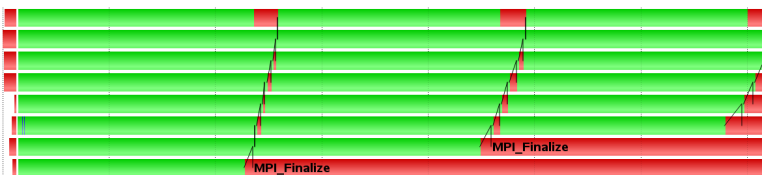
(B) Vampir trace for LB2. The Parareal runtime is R_{pa} = 5.436 (s).
