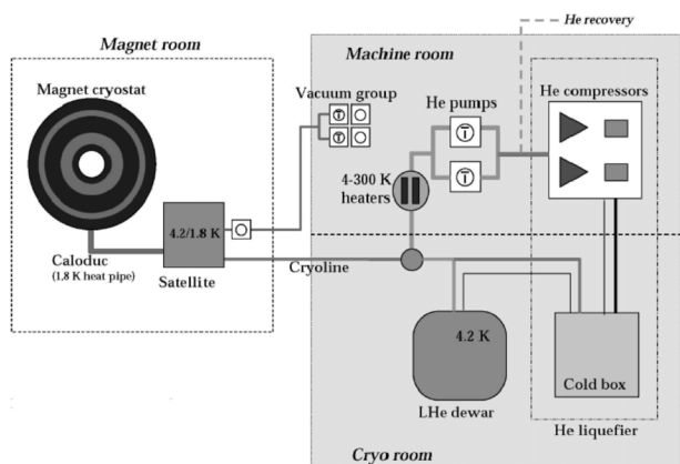
Figure 20. NeuroSpin general layout with the superfluid helium heat pipe [32].
