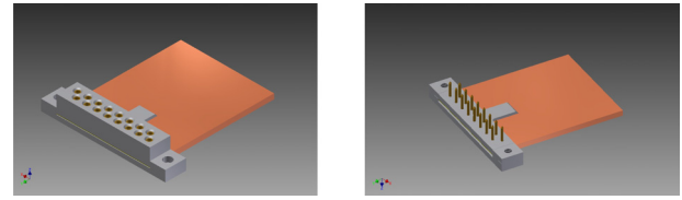
Figure 15. The Kapton/Apical cabling with connectors – plug and socket – attached. Any of the components are made internally and thus full control over radio-purity levels can be exercised by the EURECA collaboration.
