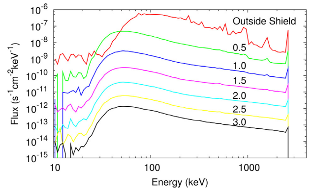
Figure 7. Gamma-ray spectra from the Th decay chain contained in the concrete of the laboratory walls attenuated by different thicknesses of water shielding (given in metres).
