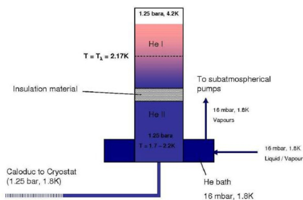
Figure 22. Claudet bath principle.
