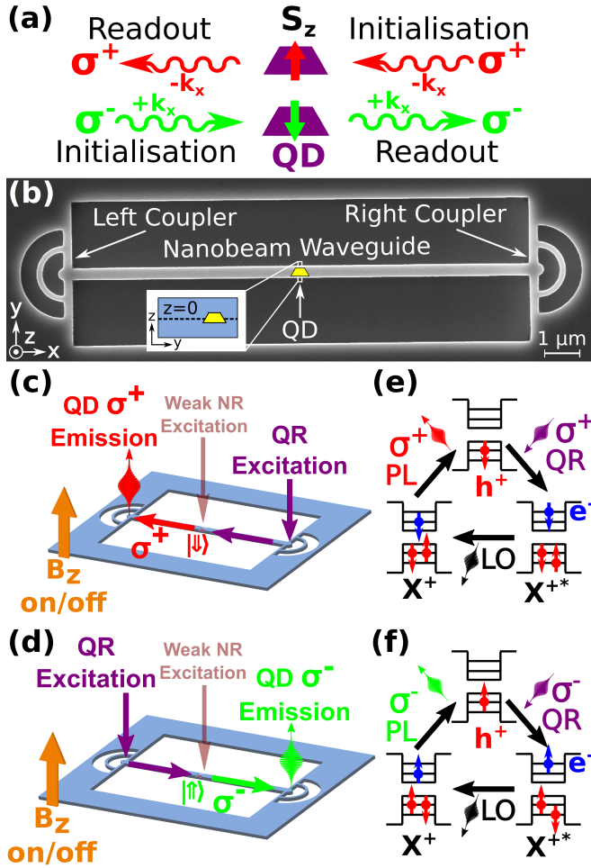
FIG. 1. (color online). (a) Schematic illustrating the relationship between photon polarization ( \sigma^+ , \sigma^- ), propagation direction ( -k_x , +k_x ), and trion pseudospin ( \uparrow , \downarrow ) for optical readout and initialization of a quantum dot spin at a chiral point. (b) Scanning electron microscope image of the device. (inset) Schematic cross-section of the waveguide. (c) and (d) Schematic of the experimental arrangement for QD exciton spin initialization from the (c) right and (d) left coupler. The QD is located at a chiral point in the waveguide. (e) and (f) Schematics showing the excitonic species involved in quasi-resonant (QR) excitation of the X^+ transition for (e) \sigma^+ (f) \sigma^- polarised excitation and emission. The Longitudinal Optic Phonon is denoted as LO.
