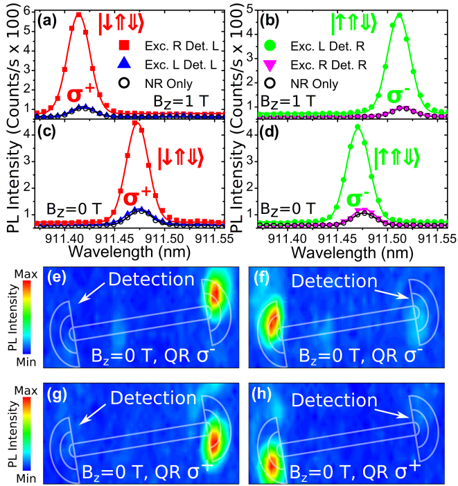
FIG. 2. (color online). (a)-(b) PL spectra obtained at B_z = 1 T when quasi-resonantly exciting the QD from each grating coupler with detection fixed at the (a) left and (b) right coupler. (c)-(d) PL spectra as in (a),(b) but with B_z = 0 T. The legends in (a) and (b) refer to the couplers on which the QR excitation laser and PL detection were located respectively (L=left coupler, R=right coupler). Spectral data are shown as solid and hollow symbols, with Gaussian fits as solid lines. Spectra with only the weak NR laser applied are shown as hollow circles. (e)-(f) Excitation maps obtained by performing a raster scan of the \sigma^- polarized QR laser over the device whilst keeping detection fixed at the (e) left and (f) right coupler. (g)-(h) Excitation maps as in (e),(f) but with \sigma^+ laser polarization. All maps recorded PL emission filtered at the QD wavelength at B_z = 0 T and a schematic outline of the waveguide and couplers are overlaid. The apparent rotation of the device from horizontal is due to a small rotation induced by the detection optics.
