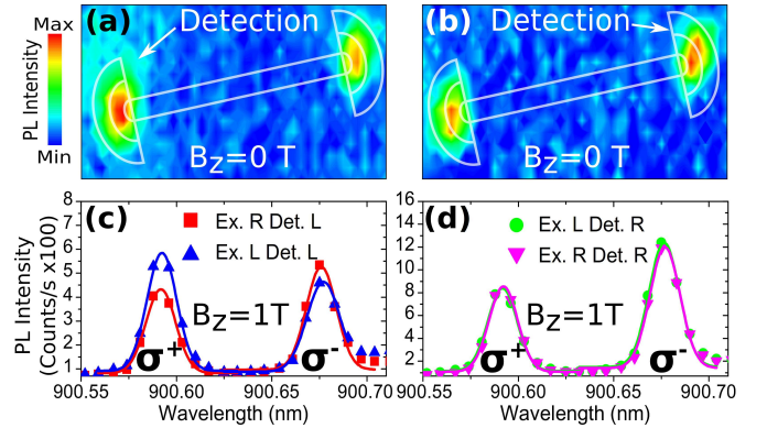
FIG. 3. (color online). (a)-(b) Excitation maps obtained by a raster scan of QR excitation over a device containing a non-chirally coupled QD whilst keeping detection fixed at the (a) left and (b) right grating couplers at B_z = 0 T. All maps recorded PL emission filtered at the QD wavelength and a schematic outline of the waveguide and couplers is overlaid. As in Fig. 2, the apparent rotation of the device from horizontal is due to a small rotation induced by the detection optics. (c)-(d) Corresponding PL spectra obtained when exciting the QD from each coupler with detection fixed at the (c) left and (d) right coupler when an external magnetic field of B_z = 1 T is applied. Spectral data are shown as solid symbols, with an experimental Gaussian fit to the data shown as a solid line.
