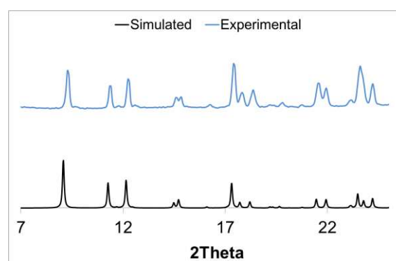
Figure 7 Powder X-ray diffractograms of Ru 12 L 2 complex 18 showing simulated trans geometry (blue) and experimental data (black).
