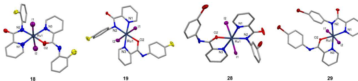
Figure 5 Molecular structures of Ru 12 L 2 complexes 18 , 19 and 28 showing trans(X)-trans(N,N)-trans(N,O) arrangements and 29 showing a trans-cis-cis arrangement. Hydrogen atoms and solvent molecules are omitted for clarity and displacement ellipsoids are at the 50% probability level (shown only for the heteroatoms).
