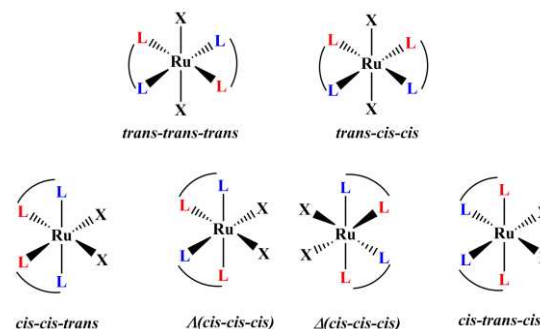
Figure 3 Possible structural isomers for ruthenium complexes of the type RuX 2 L 2 ; enantiomers for cis-cis-cis structure are also shown.
