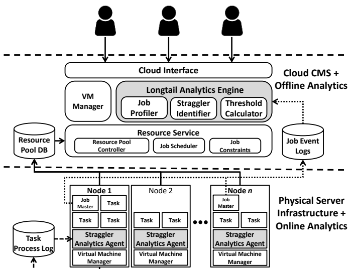
Fig 7. Cloud datacenter model with integrated Long Tail analytics engine and agent based analytics.
