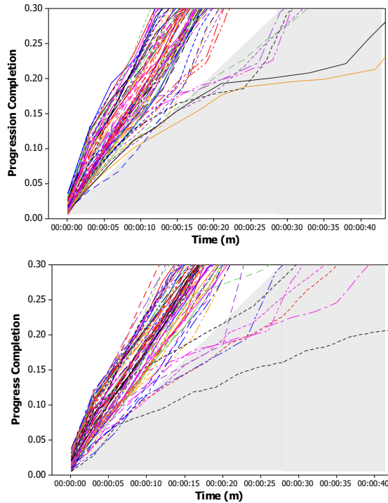
Fig 11. Threshold boundary sensitivity.
