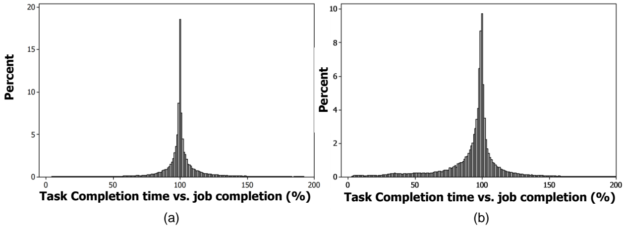
Fig 1. Google Datacenter task - job completion difference % (a) median, (b) mean.
