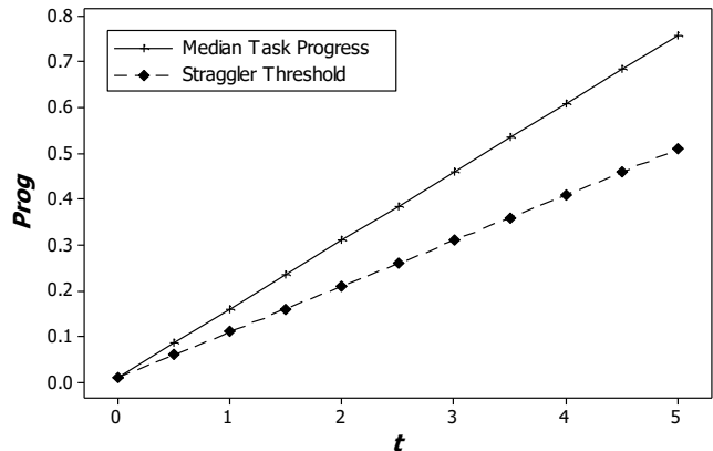
Fig 9. Representation of median task progress ( T_{iProg} ) and straggler threshold ( T_{iS} ) at time t .
