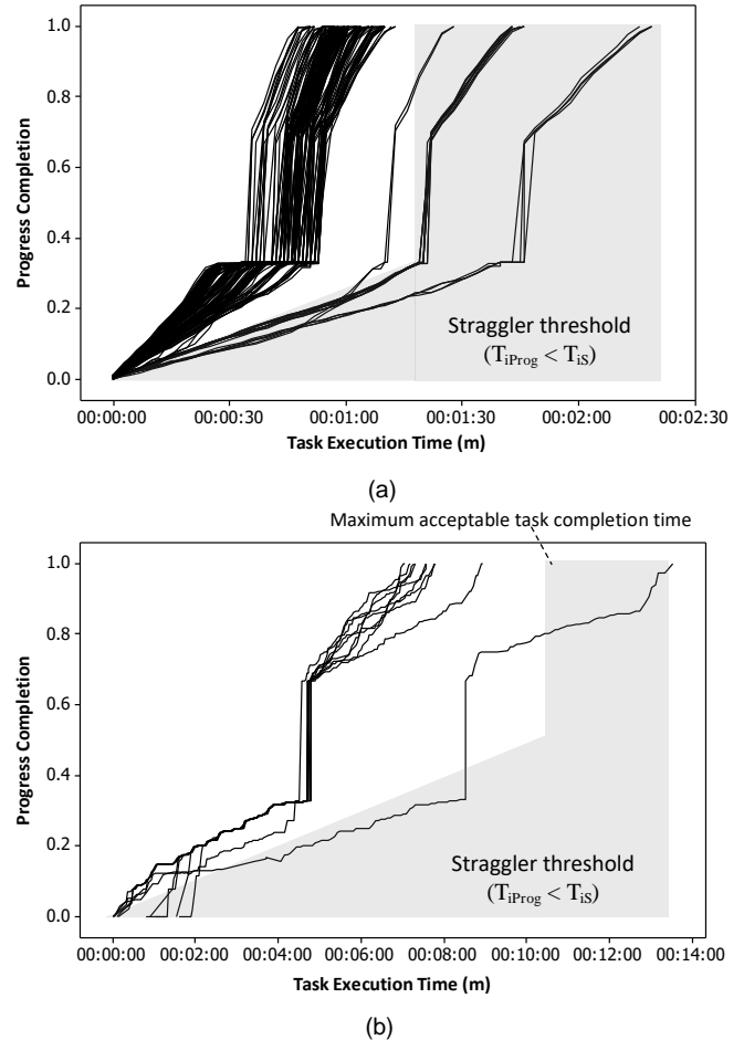
Fig 10. Task Progress with Long Tail Identification Analytics Engine (a) HiveQL, (b) WordCount.
