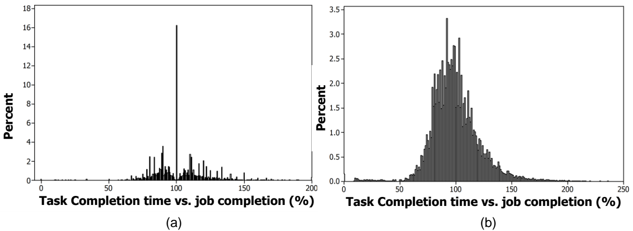
Fig 2. Cloud Datacenter B task - job completion difference % (a) median, (b) mean.
