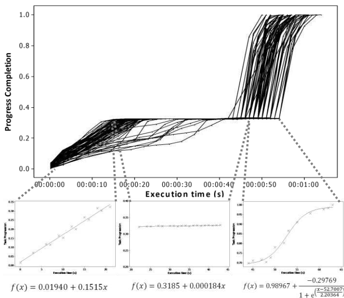
Fig 8. Example of converting empirical task progression into regression models for task progress execution.
