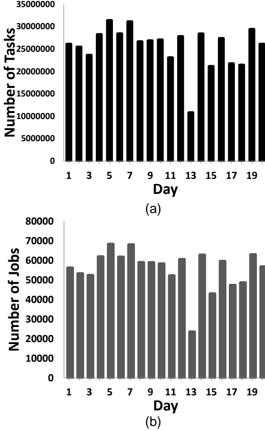
Fig 5. Workload statistics for Cloud Datacenter B (a) Tasks, (b) Jobs.
