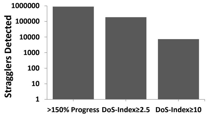
Fig 6. Number of stragglers detected with approaches.
