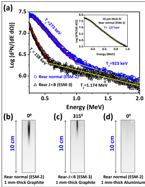
FIG. 2. Electron spectra at the rear side of the graphite target along (a) the target normal direction (blue circles) and (b) the laser propagation or J \times B direction (black triangles). Corresponding raw ESM-traces are shown in (b) and (c). Similar measurements with 1 \text{ mm} -thick aluminium target could not detect any signal above the threshold level, as shown in (d). Inset in (a) shows the rear side electron spectrum for a 10 \mu\text{m} -thick aluminium
