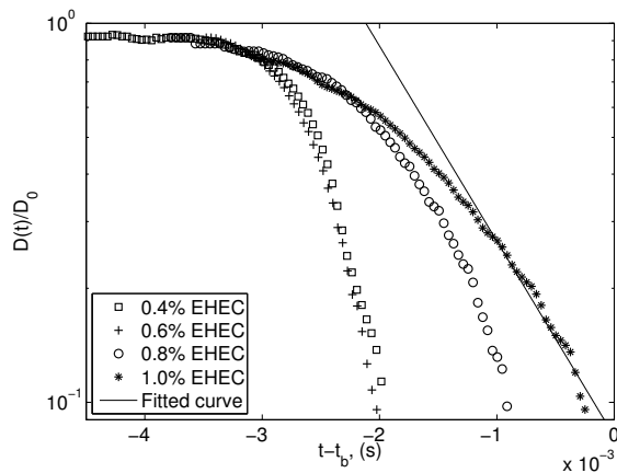
FIG. 8. The EHEC filament thinning curve as a function of time, D(t) . ( \square ) - 0.4 % EHEC, (+) - 0.6 % EHEC, ( \circ ) - 0.8 % EHEC, (*), - 1 % EHEC, solid line - fitting line for 1 % EHEC. The EHEC 0.4 %, 0.6 % and 0.8% curves are time shifted.
