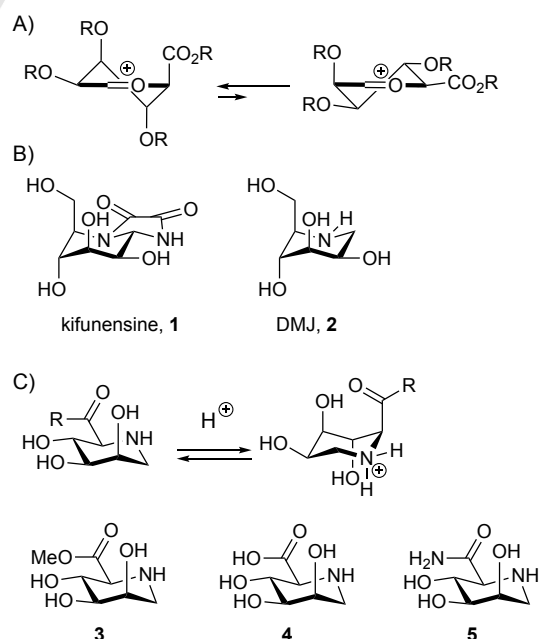
Figure 1. A) Conformational equilibrium for the mannuronic acid oxocarbenium ion. B) Structures of the mannosidase inhibitors kifunensine (1) and 1-deoxymannojirimycin (DMJ, 2) in their 1 C 4 conformation. C) Mannuronic acid azasugars studied here.
