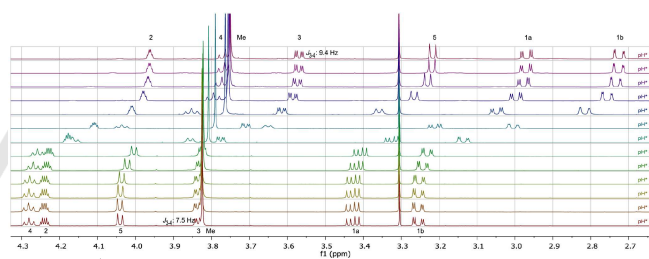
Figure 3. {}^1H NMR spectra for 2,6-dideoxy-2,6-imino-mannuronic acid methyl ester (3) at different pH*; spectra are referenced to residual methanol.
