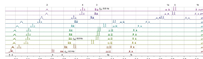
Figure 4. {}^1H NMR spectra for 2,6-dideoxy-2,6-imino-mannuronic acid (4) under different pH*; spectra are referenced to water.
