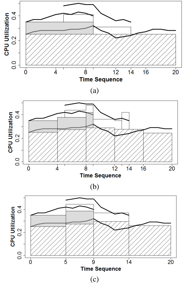
Figure 4. Visual depiction of resource boxing algorithms (a) Time zero, (b) event-based, (c) interval-based
