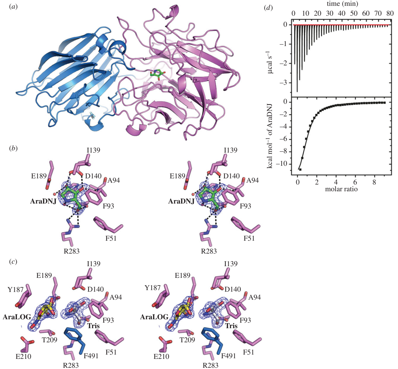
Figure 3. Overall structure and inhibitor binding to BoGH43A \alpha -L-arabinofuranosidase. (a) Overall structure of BoGH43A ; the N-terminal catalytic domain is coloured purple and C-terminal \beta -sandwich domain is coloured blue. The location of the active site is indicated by the position of AraDNJ shown in stick representation coloured by atom type with green carbons. (b) Wall-eyed stereo view of the active site in the BoGH43A -AraDNJ complex. The final 2Fo-Fc map for the ligand is shown contoured at 1\sigma in blue. The hydrogen bonding interactions made by the inhibitor are shown as black dashed lines. (c) Wall-eyed stereo view of the active site for BoGH43A -AraLOG complex. Binding of the AraLOG inhibitor (yellow carbon atoms) was too weak to displace TRIS (white carbon atoms) from the -1 sub-site and instead occupies +1 , revealing key stacking interactions with Tyr187 and other conserved residues. (d) ITC thermogram showing the binding of AraDNJ to BoGH43A in solution giving a K_d of 35 \pm 4 \mu\text{M} .
