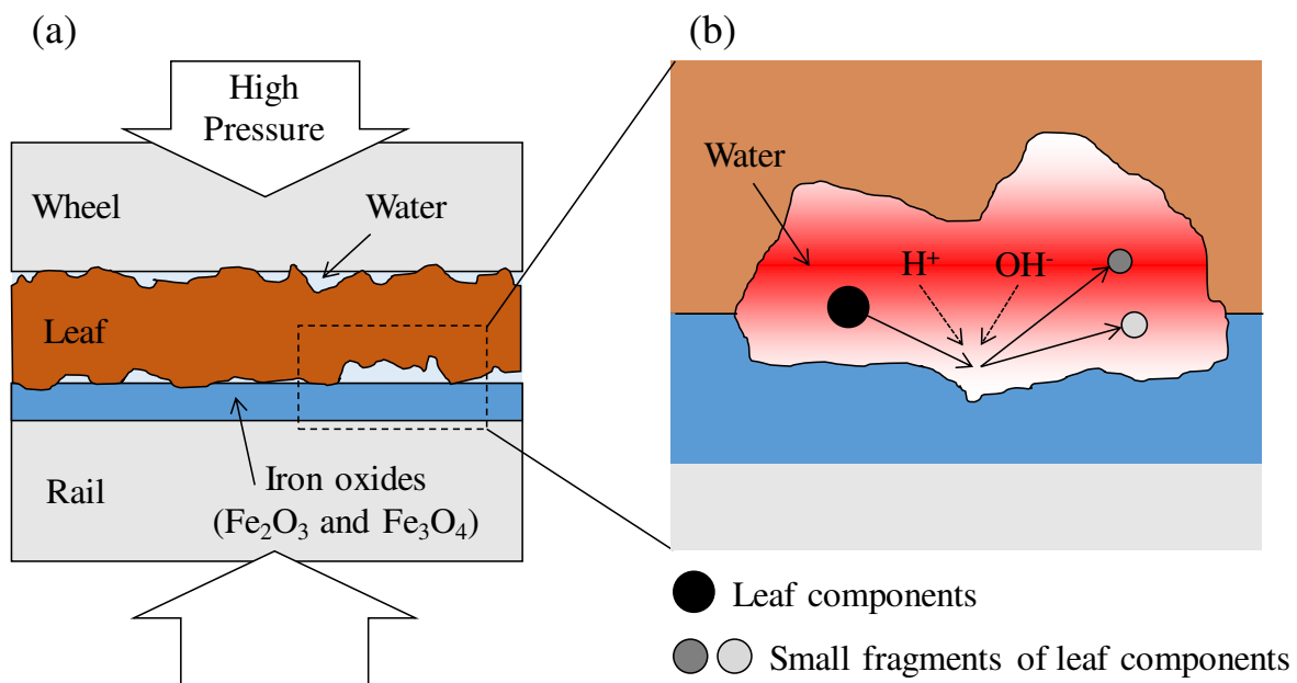
Figure 11: A decomposition process of leaf components with the catalyst of iron oxides.
