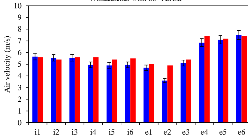
Windcatcher with 30° ASCD
