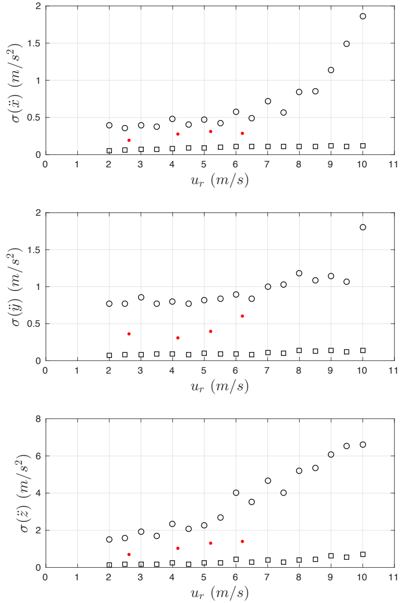
Figure 13: Standard deviations of linear acceleration data from the head sea sea-trials (red dots), h_s = 0.1\text{m} head sea simulation (black squares) and h_s = 1.25\text{m} head sea simulation (black circles), for varying relative surge velocity ( u_r ).
