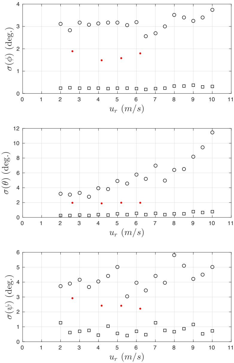
Figure 14: Standard deviations of angular displacement data from the head sea sea-trials (red dots), h_s = 0.1\text{m} head sea simulation (black squares) and h_s = 1.25\text{m} head sea simulation (black circles), for varying relative surge velocity ( u_r ).
