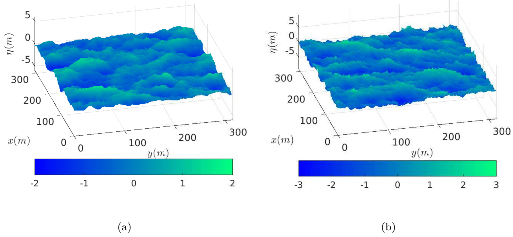
Figure 5: Sea-surface elevation plots of: (a) ocean swell produced using the EY spectrum in Figure 4(a), (b) ocean swell travelling against a surface current produced using the EY spectrum and current influence spectrum in Figure 4(b). Both plots are comprised of 512^2 waves.
