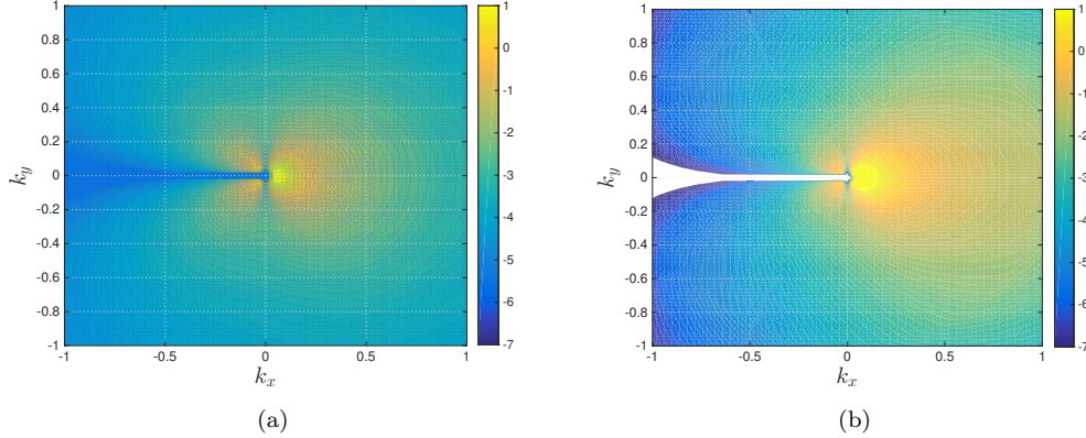
Figure 4: Contour plots of: (a) \log_{10} \Psi_{\text{EY}}(k_x = k \cos(\theta), k_y = k \sin(\theta)) for southerly swell windspeed 10m/s, 10^4 km fetch, Sea State 4 and (b) \log_{10} \Psi_{\text{EY}} for northerly surface current speed U_c = 2\text{m/s} , southerly swell windspeed 10m/s, 10^4 km fetch and corresponding to Sea State 5.
