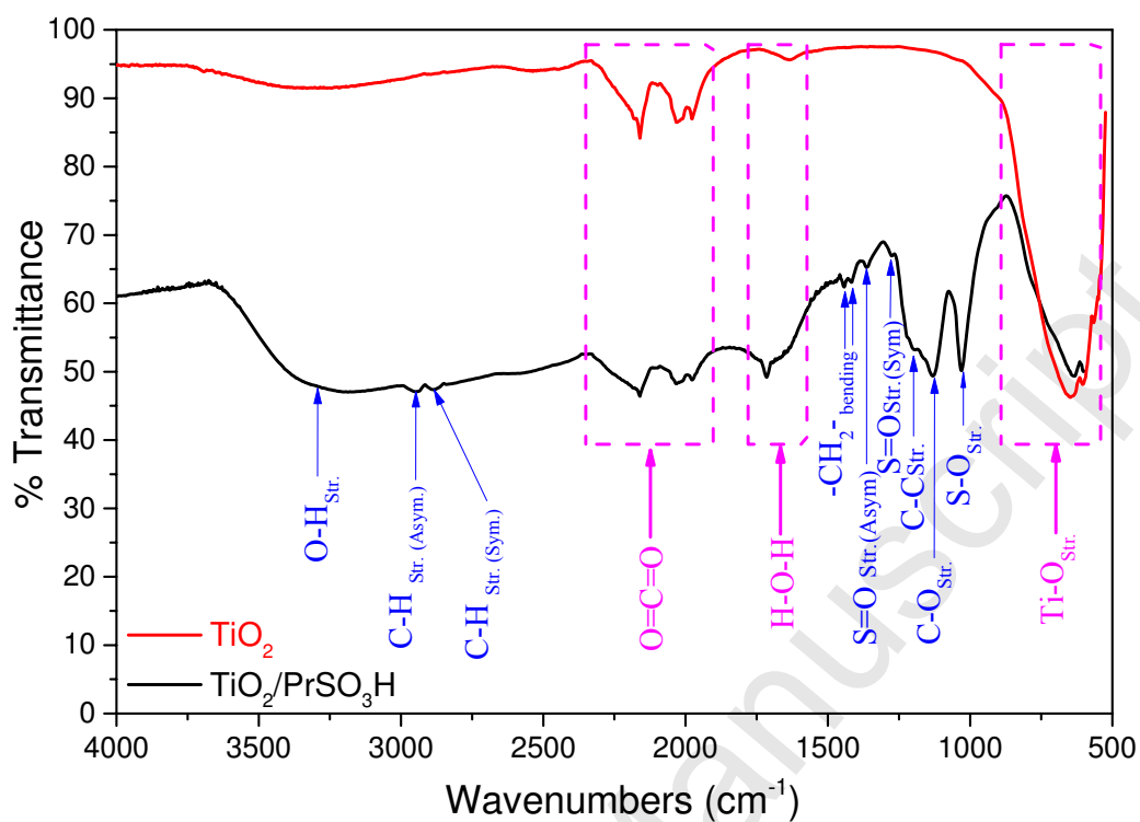
Figure (1): FT-IR spectra of \text{TiO}_2/\text{PrSO}_3\text{H} (in black) and \text{TiO}_2 (in red) nano-catalysts
