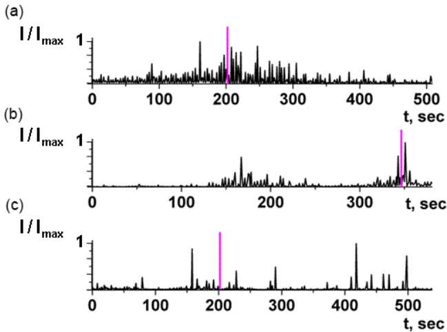
Figure 9. CE3 The intensity distribution of VLF range signals registered on board the DEMETER satellite, normalized to the corresponding maximum value: (a) and (b) after the acoustic disturbance, and (c) without the acoustic disturbance. The beginning of the acoustic radiation was chosen at a moment of time 10 min before the moment of time corresponding to the minimum distance from the satellite to the point of the acoustic generation. The vertical arrow of each plot is the moment of the minimum distance from the satellite to the point of the acoustic generation ( L_{\text{viv}} ). Panel (a) shows satellite flight over artificial acoustically disturbed zone (200 s), (b) shows satellite flight over Vrancea earthquake zone (Romania) first (130–210 s) and then over artificial acoustically disturbed zone (320–380 s), and (c) shows satellite flight over the point of the acoustic radiator location when generation is absent (200 s).
