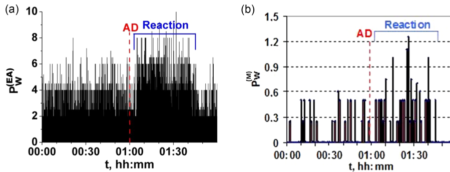
Figure 8. Time distribution of the whistler density before (00:00–01:00 UT \tau_{TS11} ) and after (01:00–02:00 UT) the acoustic disturbance. AD is the moment of acoustic disturbance. Distribution ( P_W^{(EA)} ) (Fig. 8a) was created with the superposed epoch analysis method for data from 32 experiments, carried out on different days. Distribution ( P_W^{(M)} ) \tau_{TS12} (b) was created with the median filtration method for the same data.
