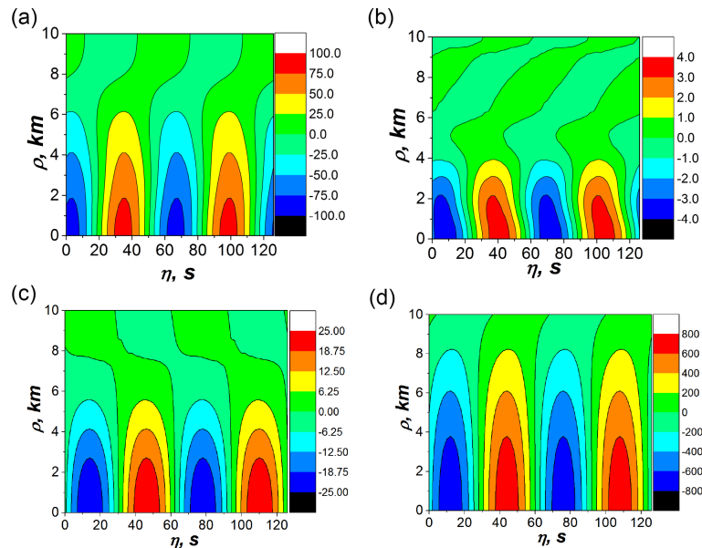
Figure 3. Spatial distribution of the air velocity v in ULF AGWs ( \text{cm s}^{-1} units) for different parameters. Panels (a), (d), and (c) are for the double frequency transforms 600 \text{ Hz} \rightarrow 25 \text{ Hz} \rightarrow 0.016 \text{ Hz} and 600 \text{ Hz} \rightarrow 100 \text{ Hz} \rightarrow 0.016 \text{ Hz} , respectively (CE6); (b) is for the single frequency transform 25 \text{ Hz} \rightarrow 0.016 \text{ Hz} . (CE7) All panels are for an initial transverse SW width of 1 and 2.5 m; panel (a) is for an initial transverse SW amplitude of 320 and (b), (c), and (d) are for one of 420 \text{ m s}^{-1} ; and panels (a) and (d) are for an altitude of Z = 300 \text{ km} and (b) and (c) are for an altitude of Z = 130 \text{ km} .
