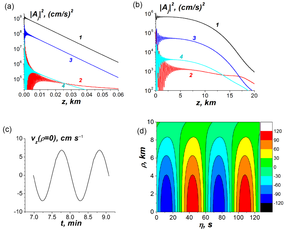
Figure 2. The double frequency transform 600\text{ Hz} \rightarrow 25\text{ Hz} \rightarrow 0.016\text{ Hz} from an initial transverse SW width of 1 m at a frequency of 600 Hz and an amplitude of 420\text{ m s}^{-1} : (a) the dependence of |A_j|^2 ( A_1 , A_2 , etc. are maximum amplitudes of harmonics at the frequency 600 Hz), (b) the dependence of |A_j|^2 (squares of the maximum amplitudes of harmonics of the intermediate frequency f = 25\text{ Hz} ) for the second transform, and (c, d) distributions of the air velocity v_z in ULF AGWs ( \text{cm s}^{-1} units) at the heights z = 130\text{ km} and z = 300\text{ km} , respectively. CES The dependence v_z(t) in the centre of the beam in panel (c) is given with an account of the time delay.
