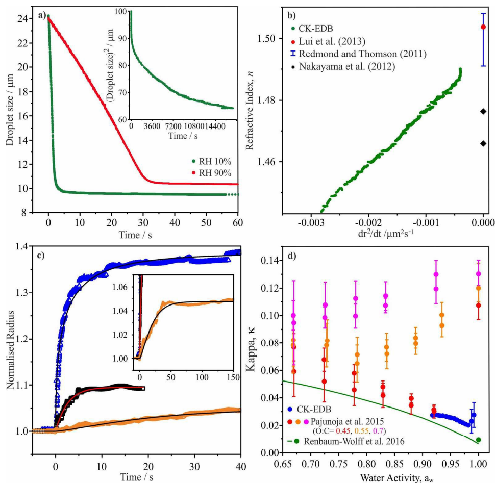
Figure 6. (a) Evaporation profile of aqueous \alpha -pinene SOA (O:C of 0.43) droplet at two RHs, inset shows long time evaporation (radius 2 vs time). (b) CK-EDB refractive index variation with dr^2/dt plotted with literature SOA measurements (dry). 9 (c) Water condensation kinetics on sodium nitrate, sucrose and aqueous \alpha -pinene SOA at 0°C, showing normalised radius. Inset shows long time condensation profile for aqueous \alpha -pinene SOA. (d) \kappa vs a_w for CK-EDB aqueous \alpha -pinene SOA at 20°C compared with literature values. 65,114
