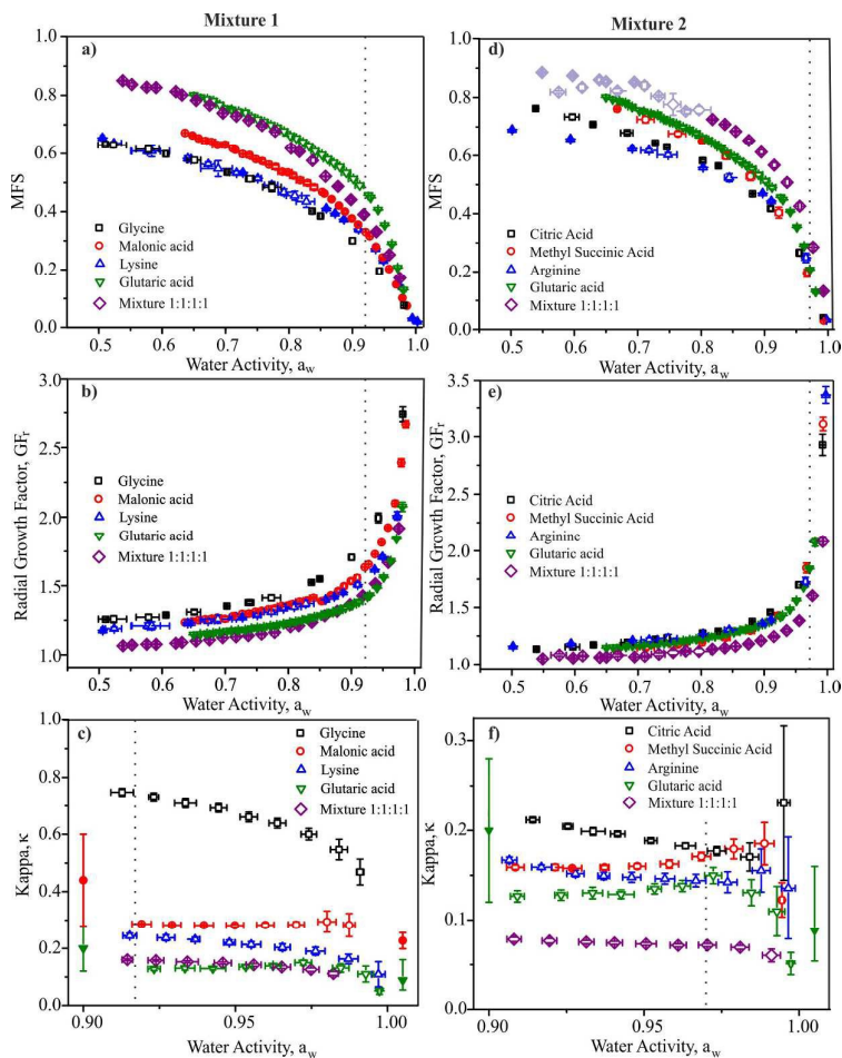
Figure 2. Mass fractions (a, d), radial growth factor (b, e) and \kappa (c, f) vs. a_w for Mixture 1 and 2, respectively at 20°C. Data for the four binary aqueous solutions are also shown for comparison. 110 Dotted lines indicate the bulk solubility limits. In (d) the light shaded purple open diamonds represent data where water transport was limited by droplet viscosity. In (c) and (f), literature data are shown (filled symbols) for glutaric acid 111,112 and malonic acid 112,113 from subsaturated (at a_w = 0.9 ) and supersaturated measurements ( a_w > 1.0 ) for comparison.
