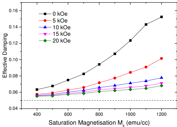
Figure 7. (Color online) Damping as a function of saturation magnetization for a range of values of the intergranular exchange, H_{\text{exch}}^{\text{sat}} .
