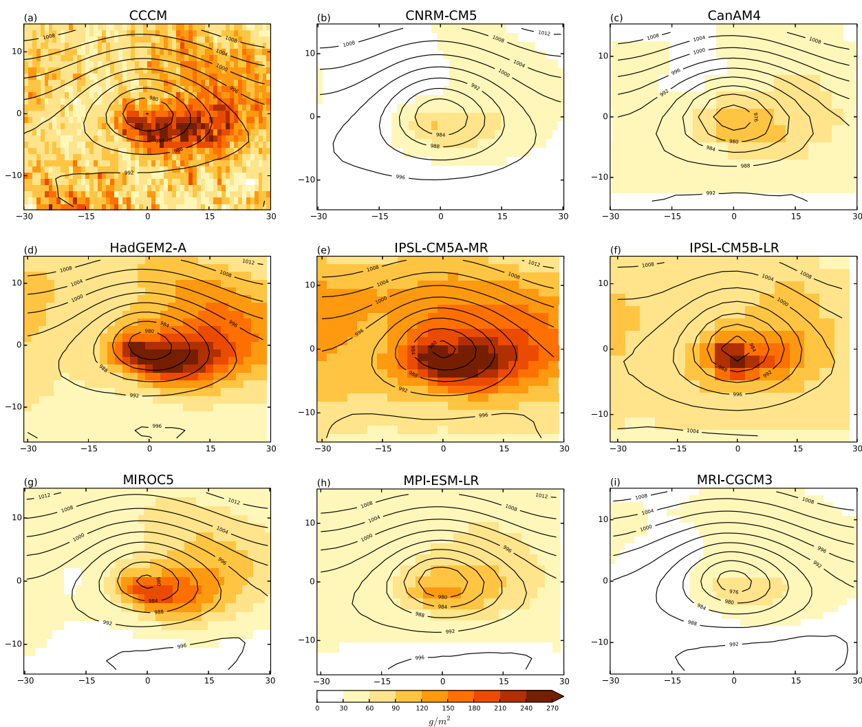
FIG. 9. As in Fig. 8, but for IWP.
